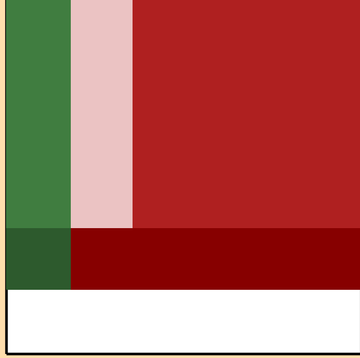
\Delta\sigma/\sigma vs. E for ^{157}\text{Pm}(n,\gamma)
