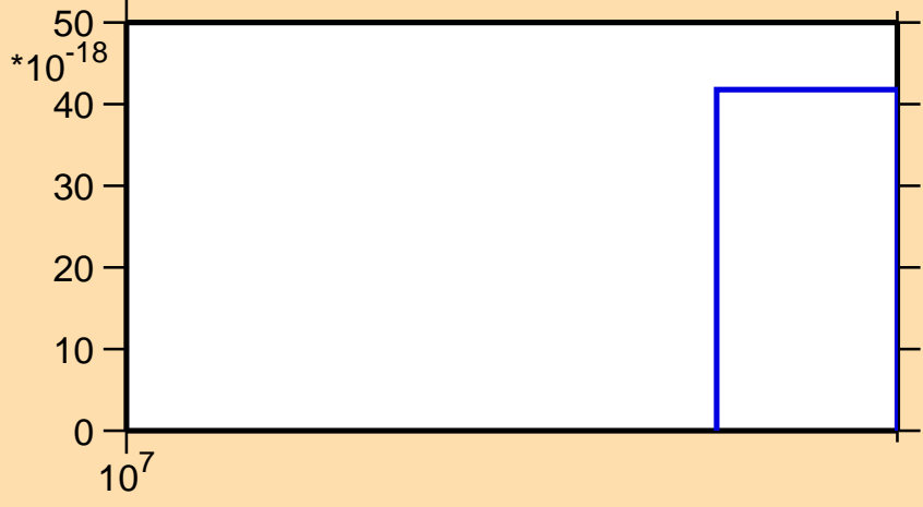
\sigma vs. E for ^{158}\text{Pm}(\text{mt } 11)
