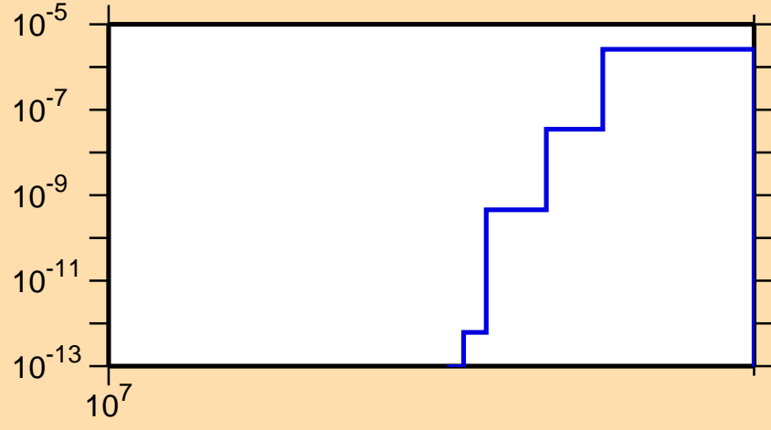
\sigma vs. E for ^{158}\text{Pm}(n,nt)
