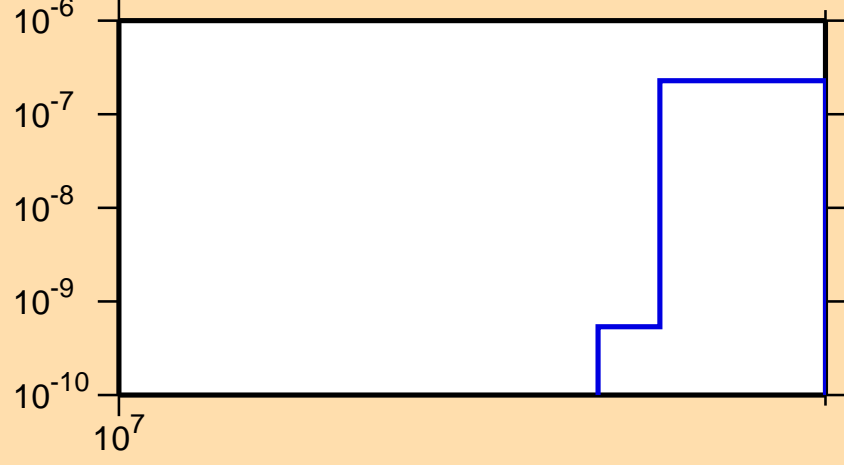
\sigma vs. E for ^{158}\text{Pm}(n,2np)
