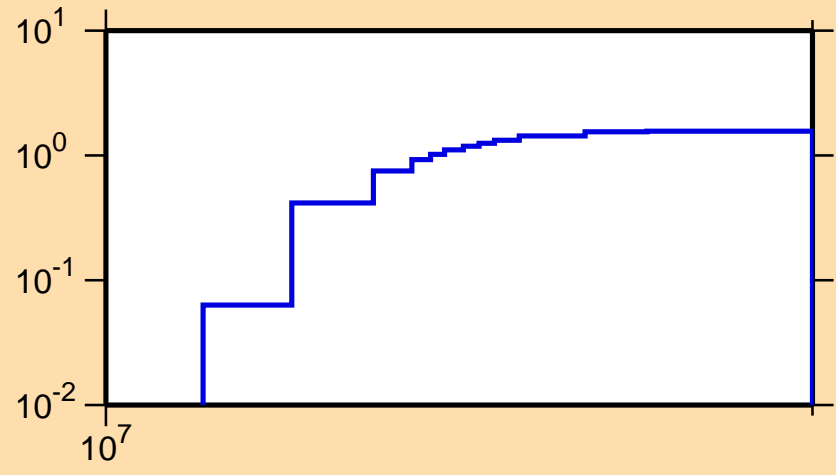
\sigma vs. E for ^{158}\text{Pm}(n,3n)
