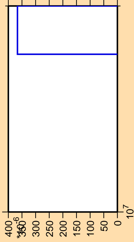
\Delta\sigma/\sigma vs. E for ^{158}\text{Pm}(\text{mt } 11)
