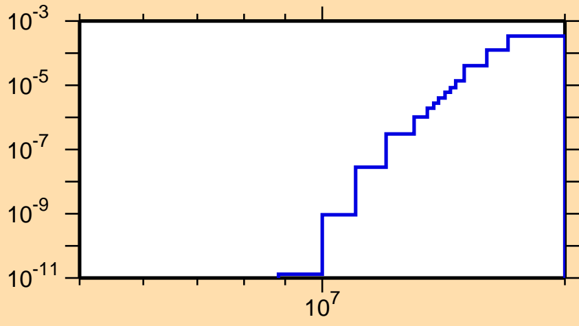
\sigma vs. E for ^{158}\text{Pm}(n,t)
