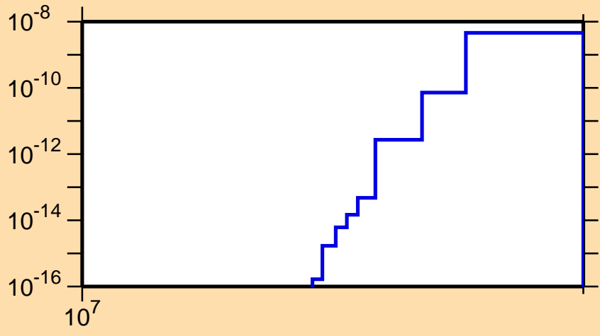
\sigma vs. E for ^{158}\text{Pm}(n,2n\alpha)
