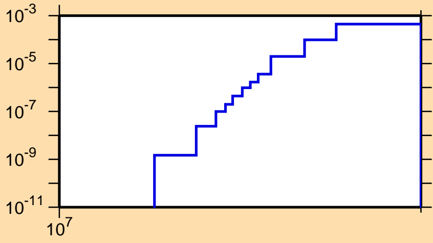
\sigma vs. E for ^{158}\text{Pm}(n,np)
