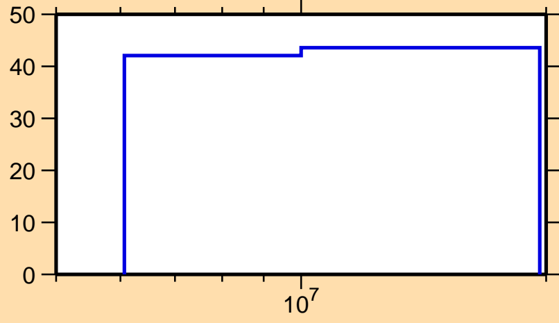
\Delta\sigma/\sigma vs. E for ^{158}\text{Pm}(n,\text{nonel.})
