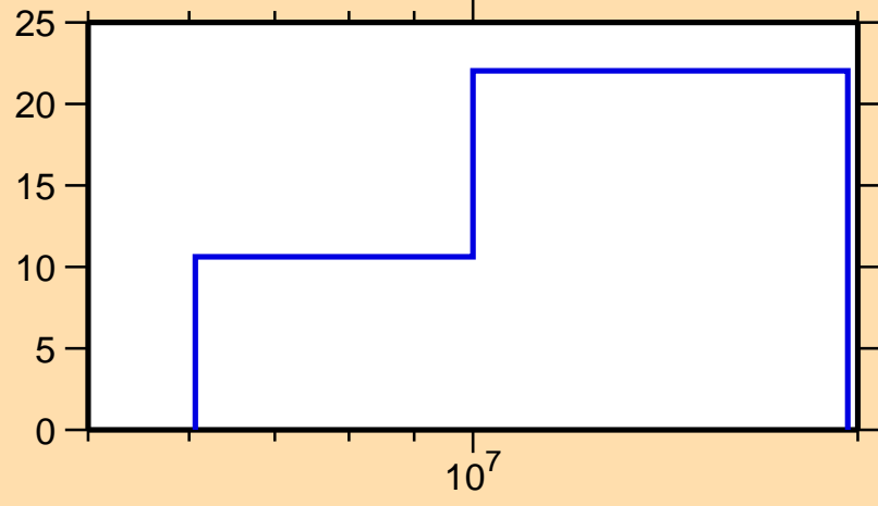
\Delta\sigma/\sigma vs. E for ^{158}\text{Pm}(n,\text{tot.})
