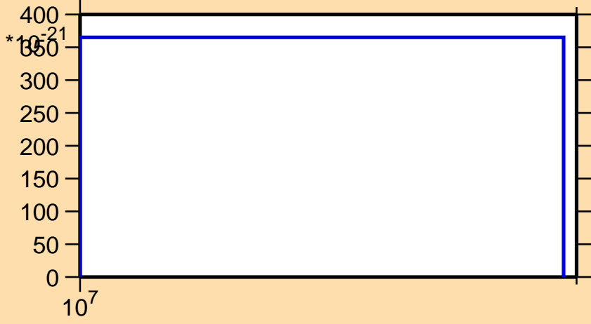
\sigma vs. E for ^{158}\text{Pm} (mt 11)
