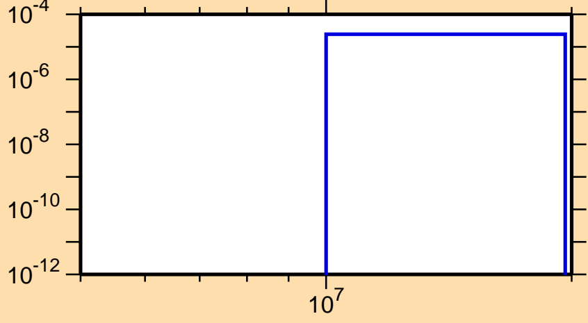
\sigma vs. E for ^{158}\text{Pm}(n,d)
