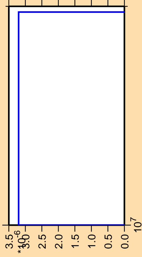
\Delta\sigma/\sigma vs. E for ^{158}\text{Pm} (mt 11)
