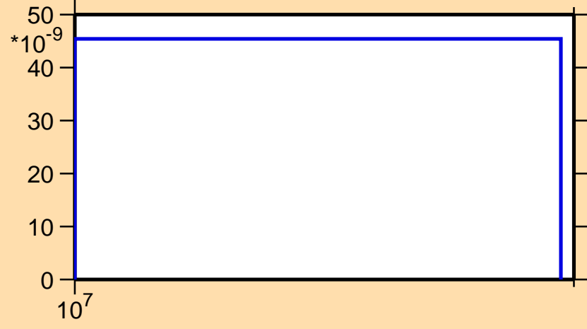
\sigma vs. E for ^{158}\text{Pm}(n,nd)
