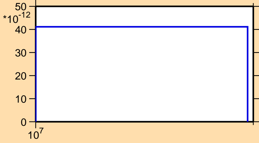
\sigma vs. E for ^{158}\text{Pm}(n,2n\alpha)
