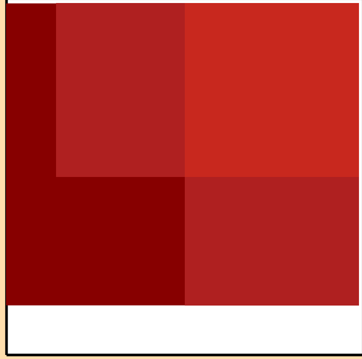
\Delta\sigma/\sigma vs. E for ^{158}\text{Pm}(n,2n)
