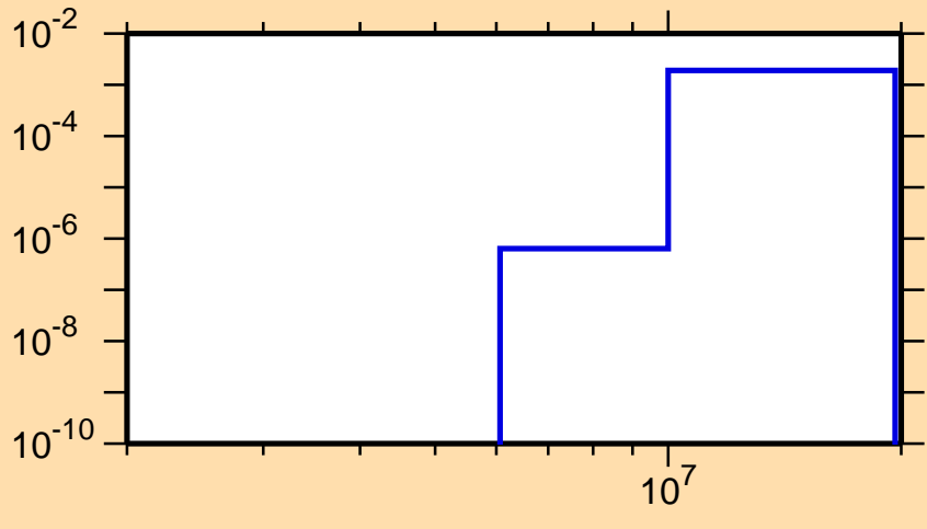
\sigma vs. E for ^{158}\text{Pm}(n,p)
