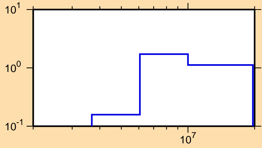
\sigma vs. E for ^{158}\text{Pm}(n,2n)
