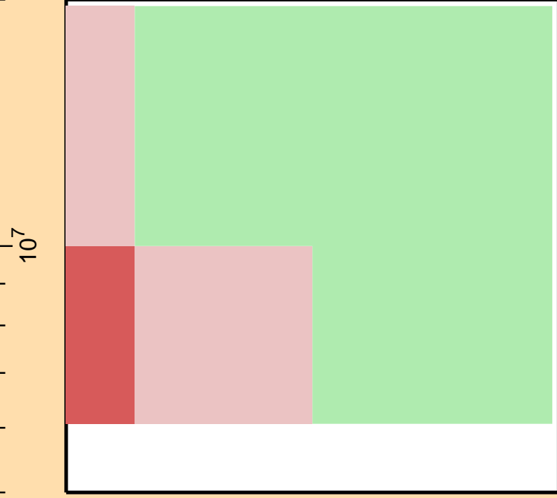
\Delta\sigma/\sigma vs. E for ^{158}\text{Pm}(n,\gamma)
