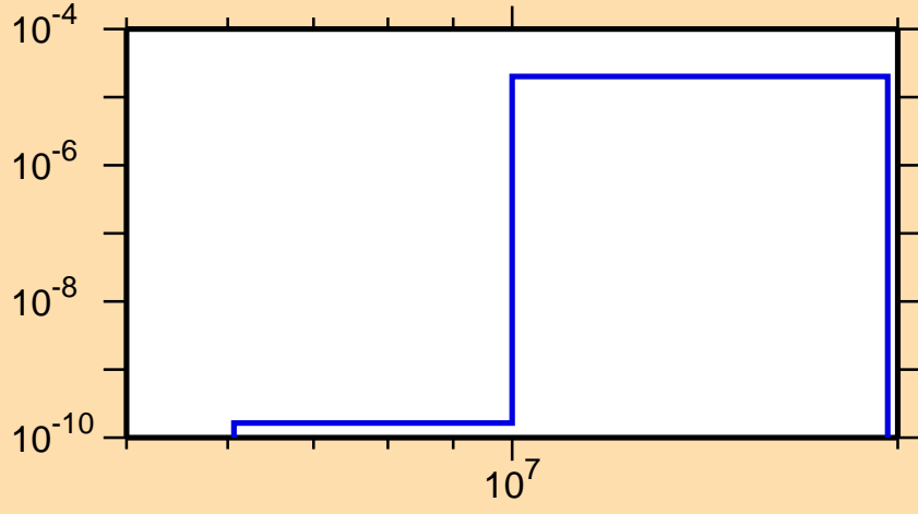
\sigma vs. E for ^{158}\text{Pm}(n,\alpha)
