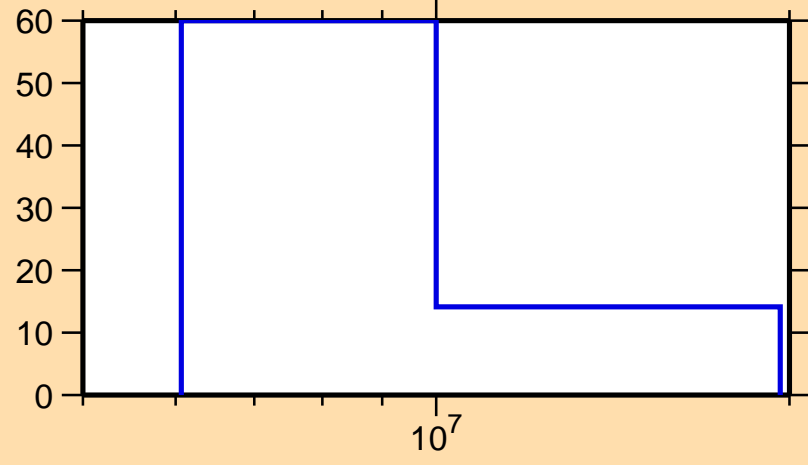
\Delta\sigma/\sigma vs. E for ^{158}\text{Pm}(n,\text{el.})
