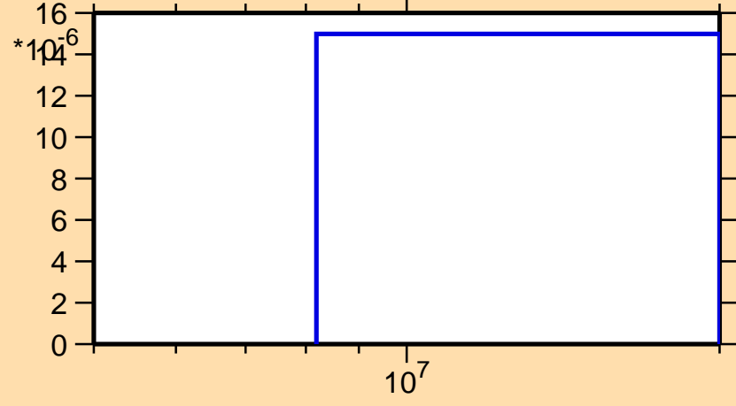
\sigma vs. E for ^{158}\text{Pm}(n,t)
