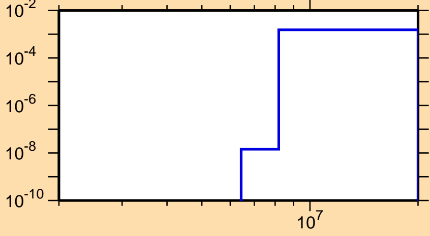
\sigma vs. E for ^{158}\text{Pm}(n,p)
