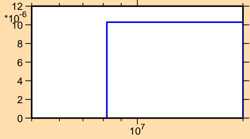
\sigma vs. E for ^{158}\text{Pm}(n,np)
