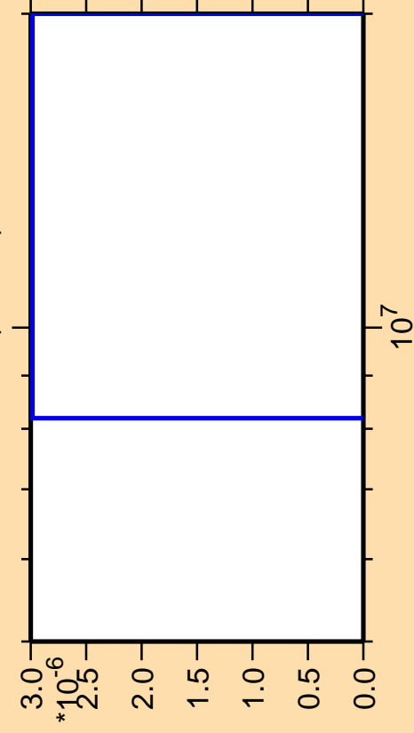
\Delta\sigma/\sigma vs. E for ^{158}\text{Pm}(\text{mt } 11)
