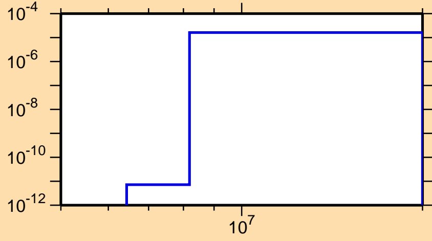
\sigma vs. E for ^{158}\text{Pm}(n,\alpha)
