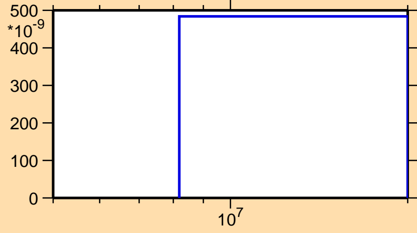
\sigma vs. E for ^{158}\text{Pm}(n,n\alpha)
