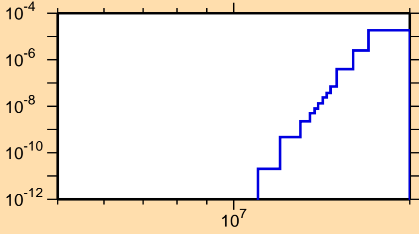
\sigma vs. E for ^{159}\text{Pm}(n,\alpha)
