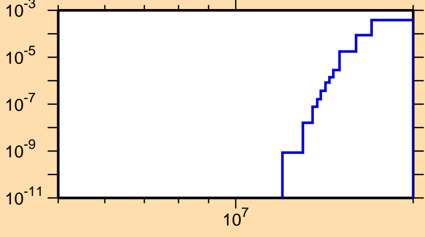
\sigma vs. E for ^{159}\text{Pm}(n,np)
