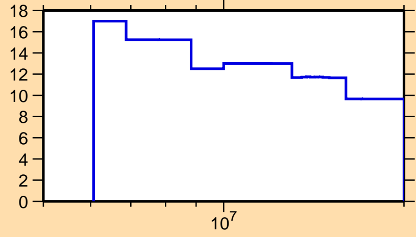
\Delta\sigma/\sigma vs. E for ^{159}\text{Pm}(n,el.)
