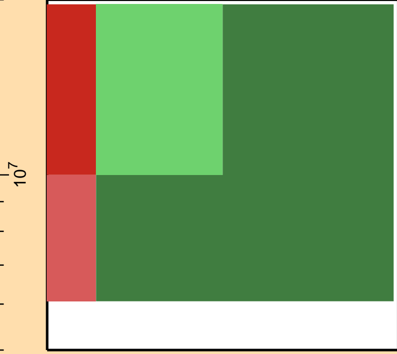
\Delta\sigma/\sigma vs. E for ^{159}\text{Pm}(n,el.)
