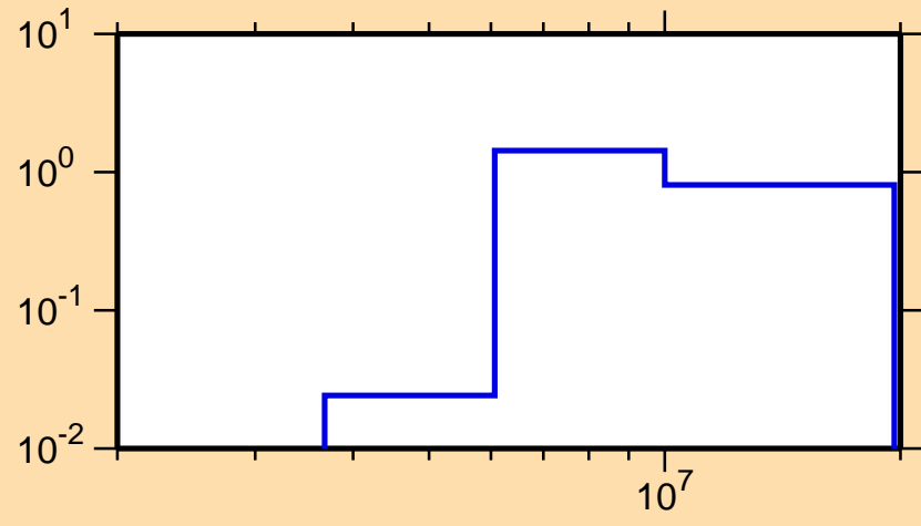
\sigma vs. E for ^{159}\text{Pm}(n,2n)
