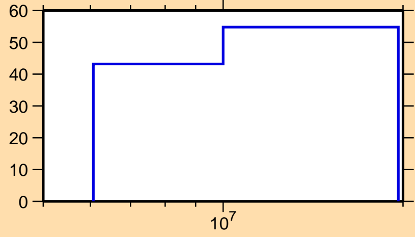
\Delta\sigma/\sigma vs. E for ^{159}\text{Pm}(n,inel.)
