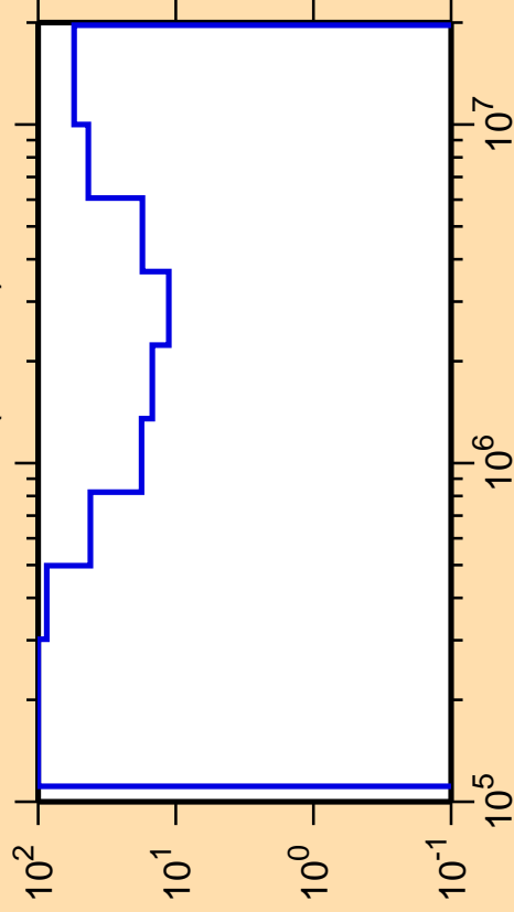
\Delta\sigma/\sigma vs. E for ^{159}\text{Pm}(n,\text{inel.})
