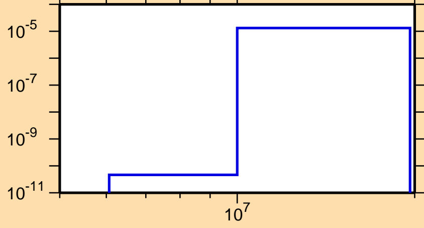
\sigma vs. E for ^{159}\text{Pm}(n,\alpha)
