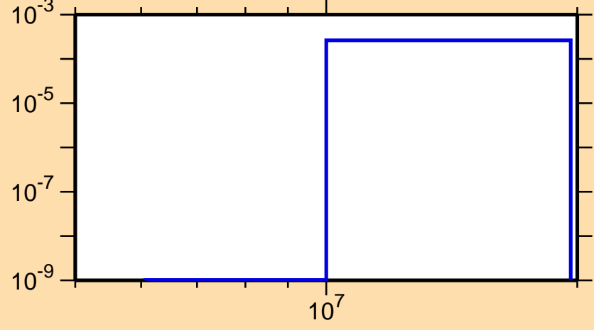
\sigma vs. E for ^{159}\text{Pm}(n,p)
