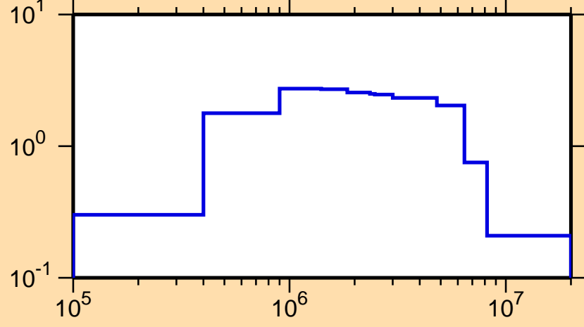
\sigma vs. E for ^{159}\text{Pm}(n,\text{inel.})
