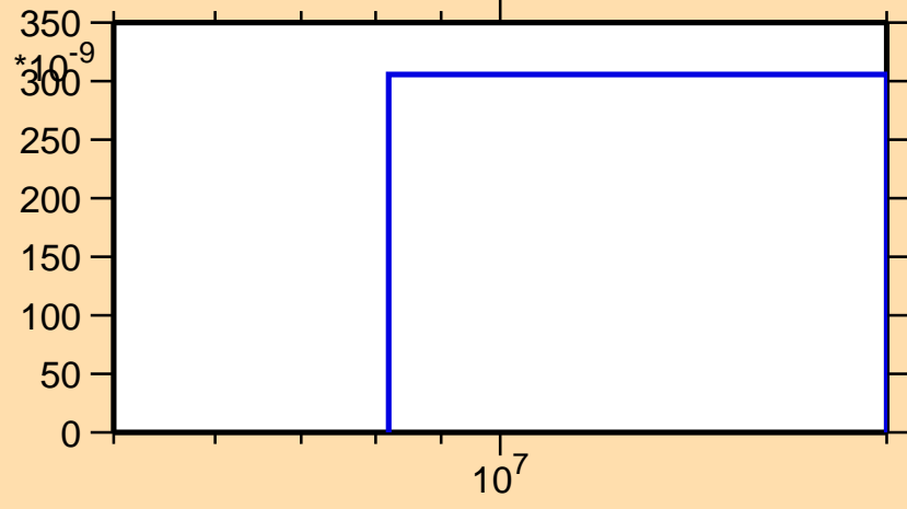
\sigma vs. E for ^{159}\text{Pm}(n,n\alpha)
