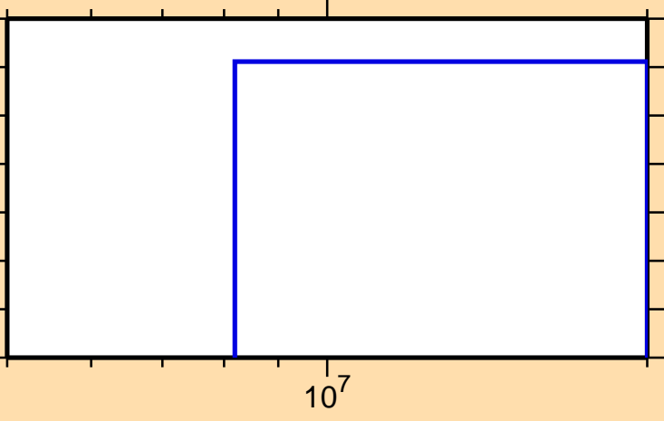
\sigma vs. E for ^{159}\text{Pm}(n,n\alpha)
