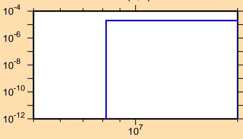
\sigma vs. E for ^{159}\text{Pm}(n,d)
