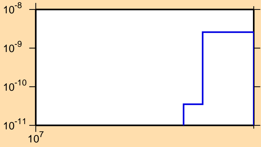
\sigma vs. E for ^{160}\text{Pm}(n,2n\alpha)
