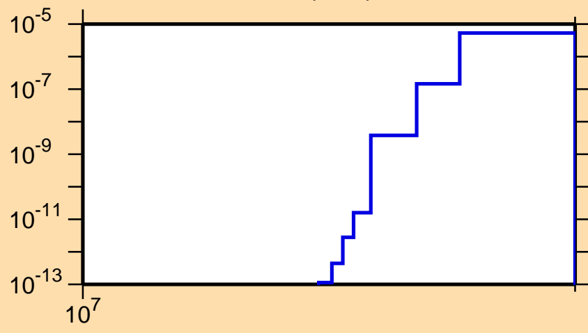
\sigma vs. E for ^{160}\text{Pm}(n,nt)
