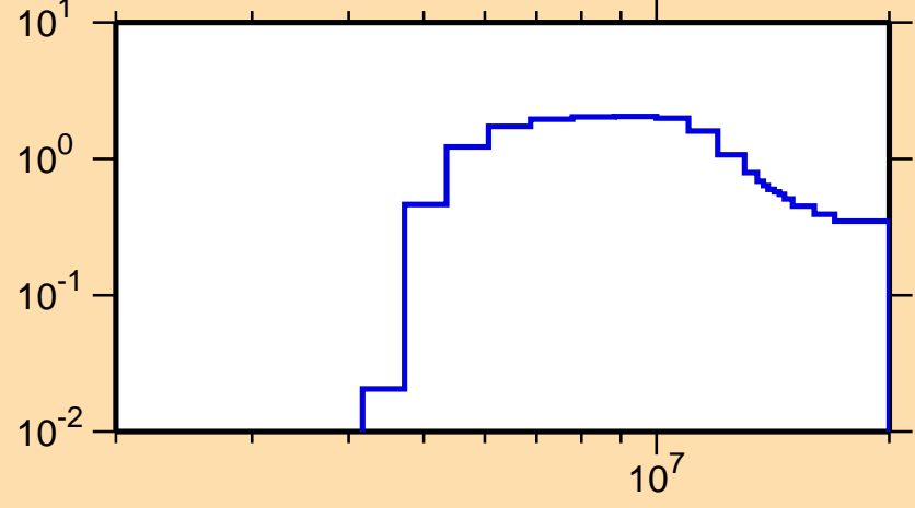
\sigma vs. E for ^{160}\text{Pm}(n,2n)
