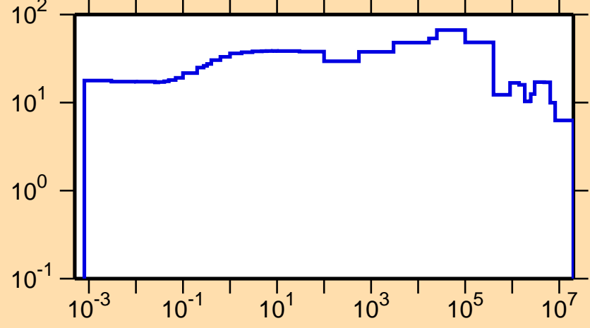
\Delta\sigma/\sigma vs. E for ^{160}\text{Pm}(n,\text{tot.})
