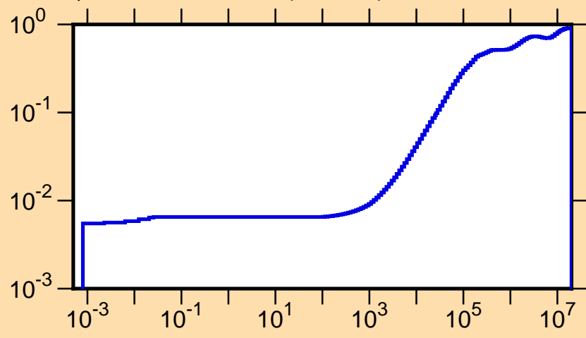
\mu vs. E for ^{124}\text{Pr}(\text{mt251})
