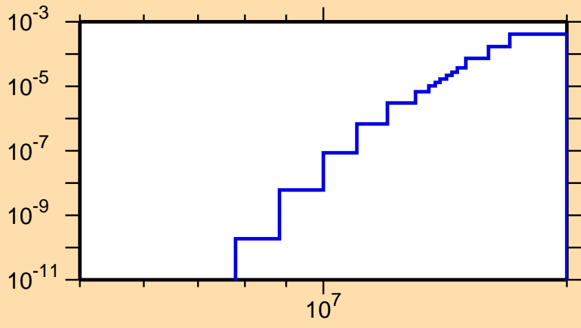
\sigma vs. E for ^{124}\text{Pr}(\text{mt } 45)
