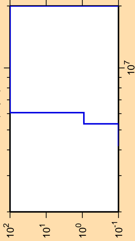
\Delta\sigma/\sigma vs. E for ^{124}\text{Pr}(n,pd)
