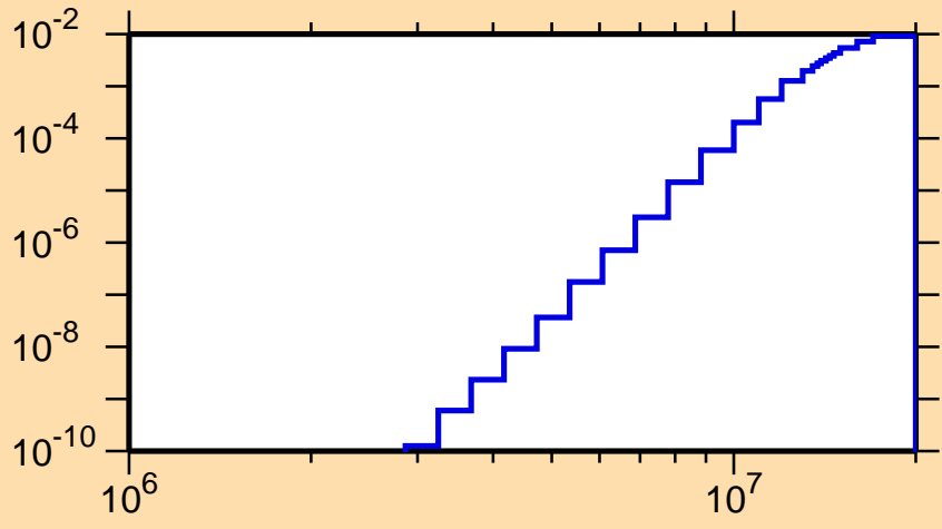
\sigma vs. E for ^{124}\text{Pr}(n,\text{He}3)
