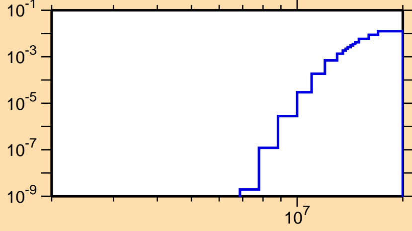
\sigma vs. E for ^{124}\text{Pr}(n,pd)
