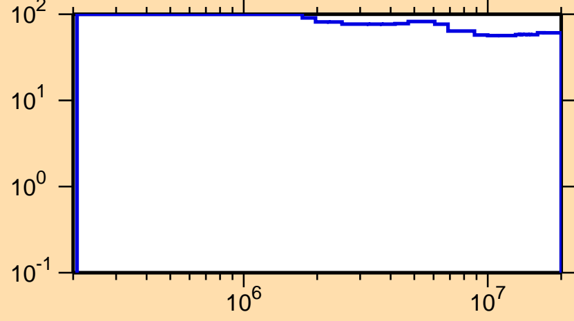
\Delta\sigma/\sigma vs. E for ^{124}\text{Pr}(n,n\text{cont.})
