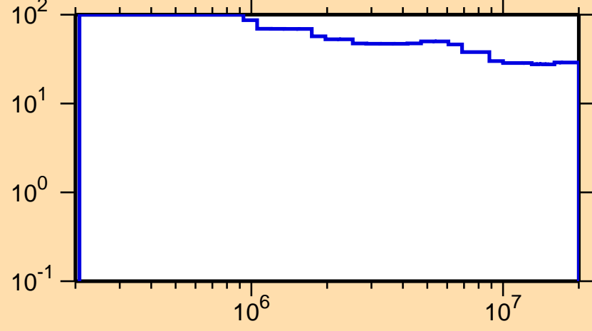
\Delta\sigma/\sigma vs. E for ^{124}\text{Pr}(n,\text{inel.})
