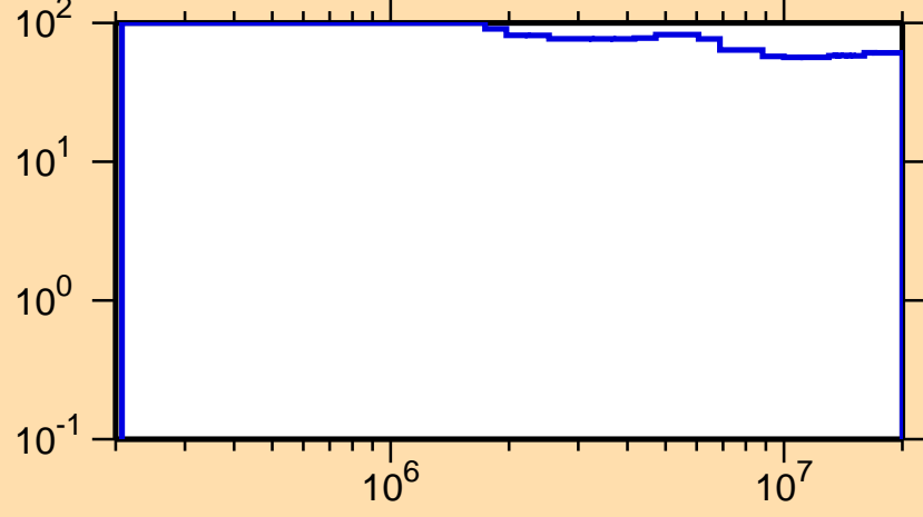
\Delta\sigma/\sigma vs. E for ^{124}\text{Pr}(n,ncont.)
