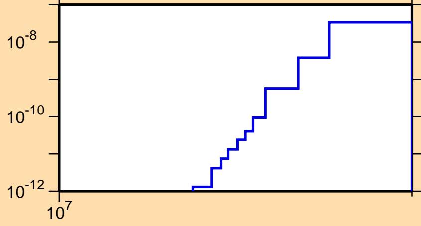
\sigma vs. E for ^{124}\text{Pr}(\text{mt } 34)
