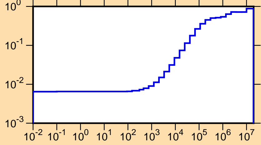
\mu vs. E for ^{124}\text{Pr}(\text{mt251})
