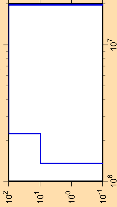
\Delta\sigma/\sigma vs. E for ^{124}\text{Pr}(n,\text{He3})
