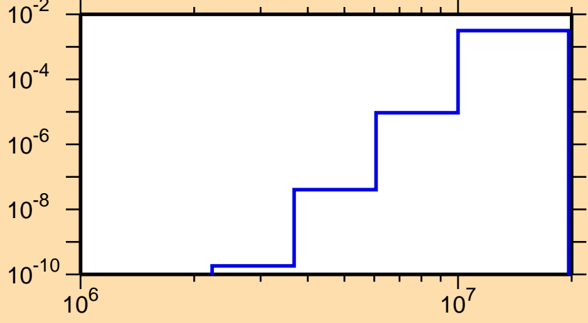
\sigma vs. E for ^{124}\text{Pr}(n,\text{He3})
