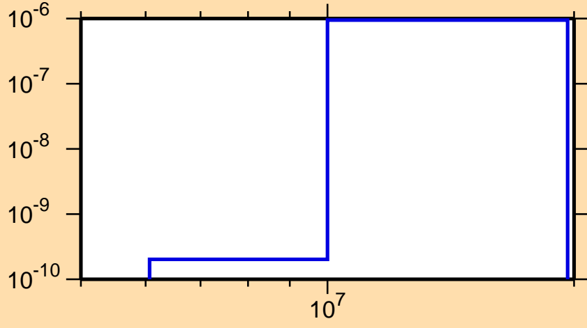
\sigma vs. E for ^{124}\text{Pr}(\text{mt117})
