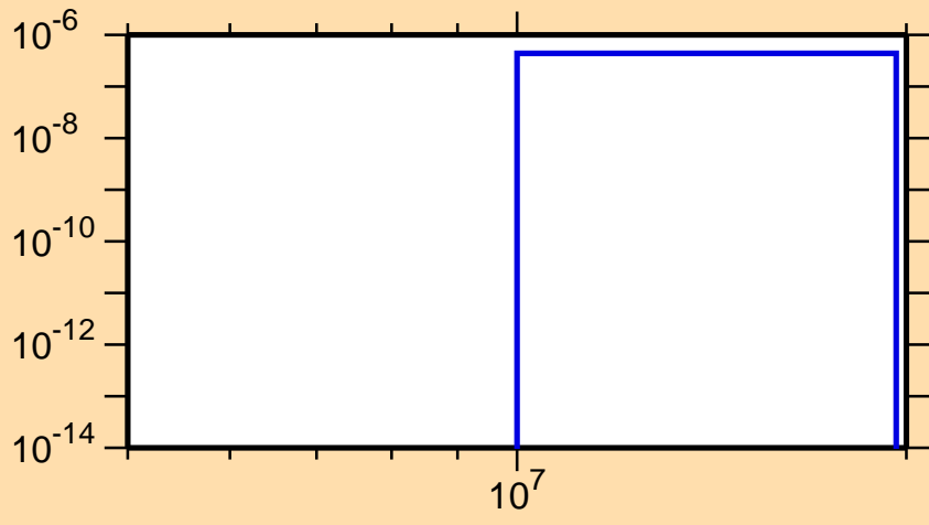
\sigma vs. E for ^{124}\text{Pr}(n,\text{nd})
