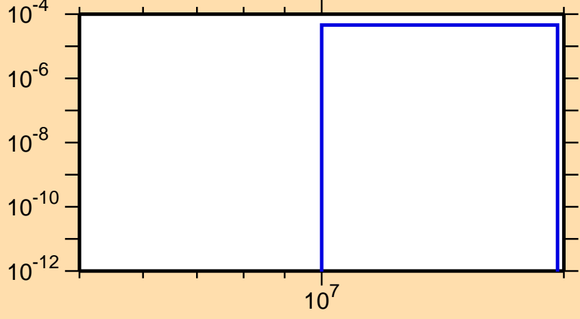
\sigma vs. E for ^{124}\text{Pr}(n,\text{pt})
