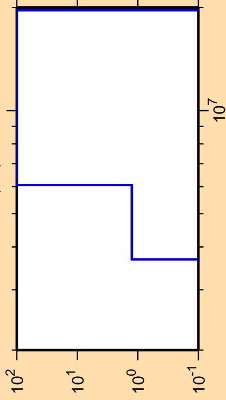
\Delta\sigma/\sigma vs. E for ^{124}\text{Pr}(n,t)
