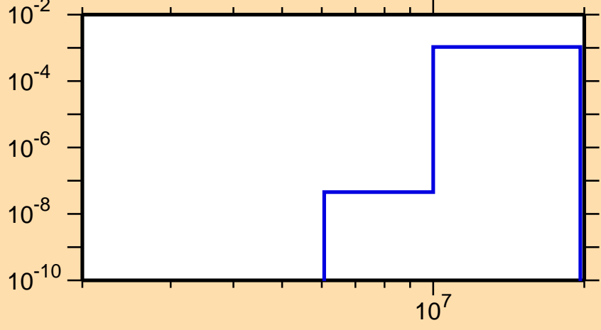
\sigma vs. E for ^{124}\text{Pr}(n,t)
