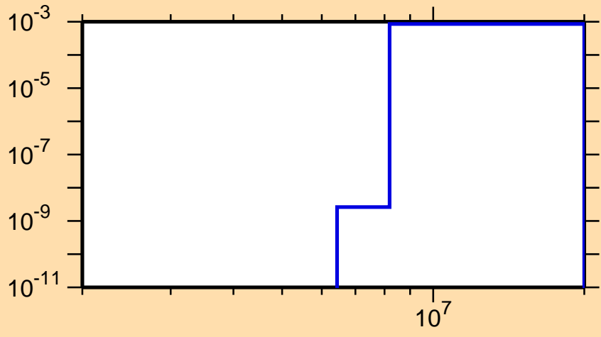
\sigma vs. E for ^{124}\text{Pr}(n,t)
