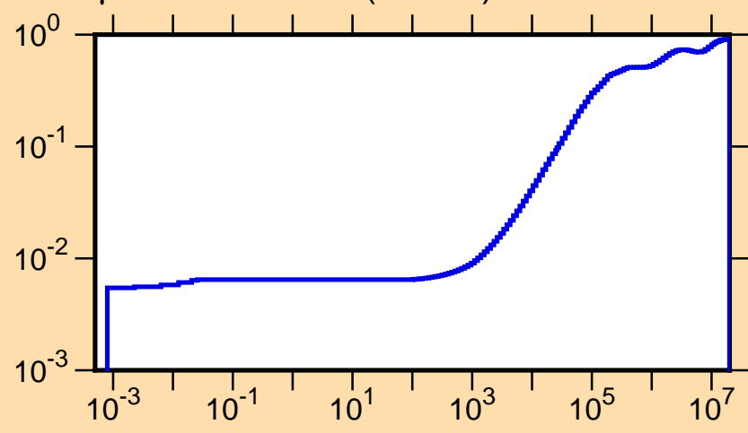
\mu vs. E for ^{125}\text{Pr}(\text{mt251})
