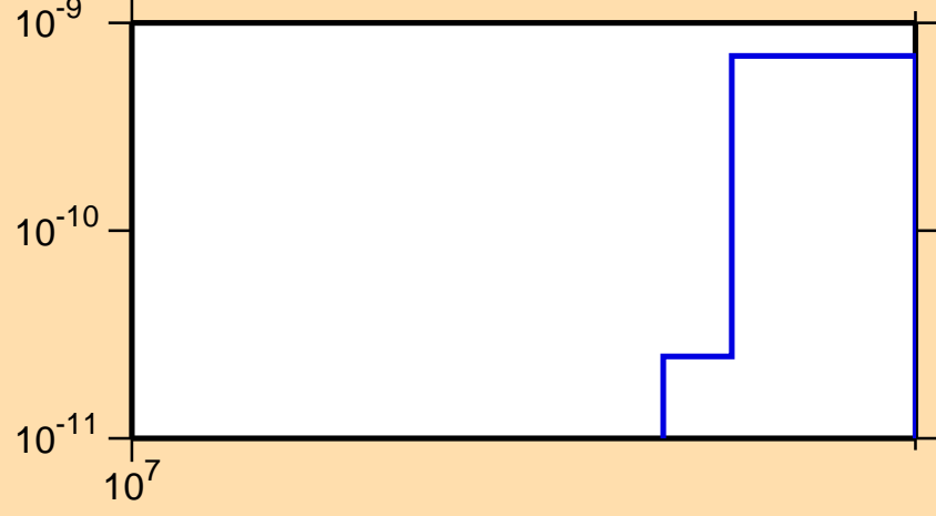
\sigma vs. E for ^{125}\text{Pr}(\text{mt } 34)
