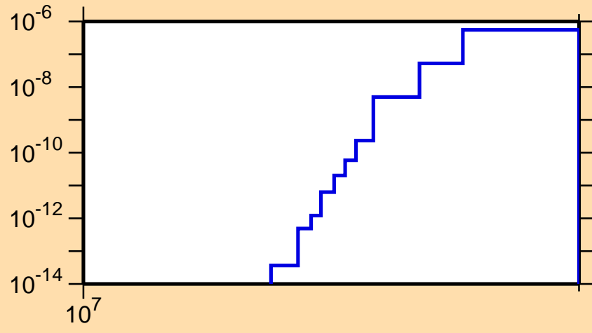
\sigma vs. E for ^{125}\text{Pr}(n,nd)
