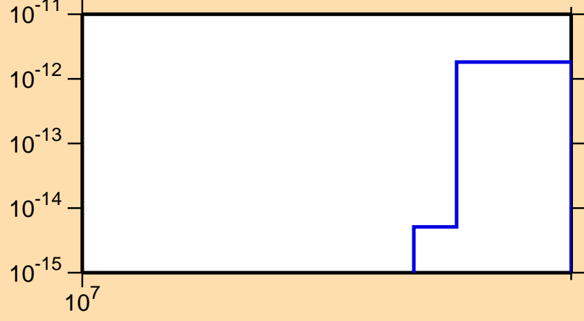
\sigma vs. E for ^{125}\text{Pr}(n,2n\alpha)
