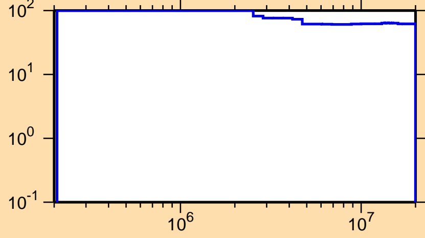
\Delta\sigma/\sigma vs. E for ^{125}\text{Pr}(n,\text{inel.})
