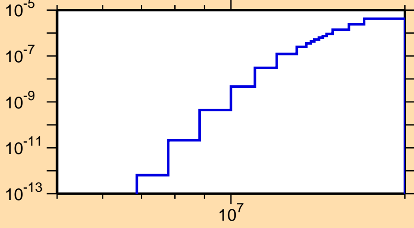
\sigma vs. E for ^{125}\text{Pr}(\text{mt117})
