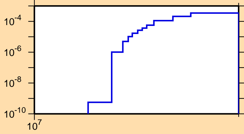
\sigma vs. E for ^{125}\text{Pr}(n,2n)
