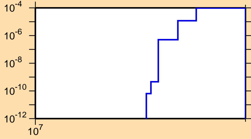
\sigma vs. E for ^{125}\text{Pr}(n,2np)
