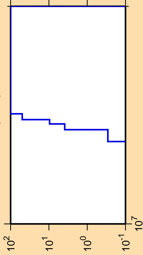
\Delta\sigma/\sigma vs. E for ^{125}\text{Pr}(n,nd)
