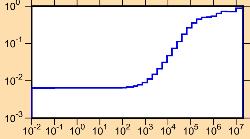
\mu vs. E for ^{125}\text{Pr}(\text{mt251})
