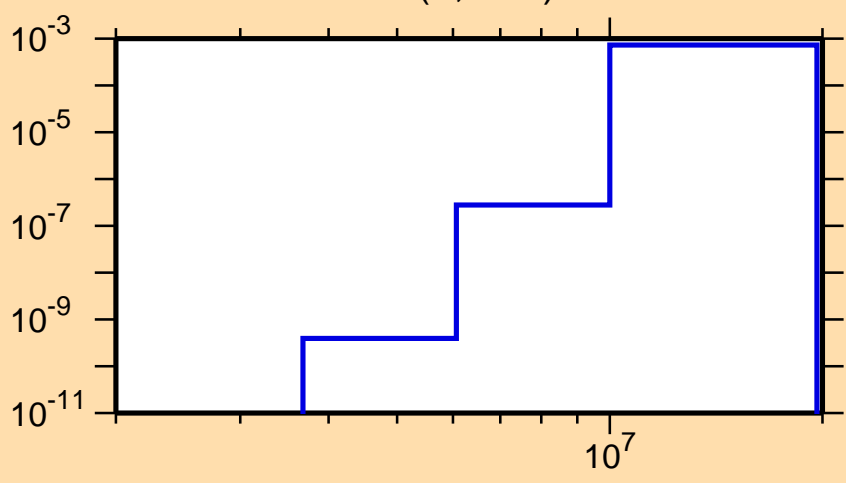
\sigma vs. E for ^{125}\text{Pr}(n,\text{He}3)
