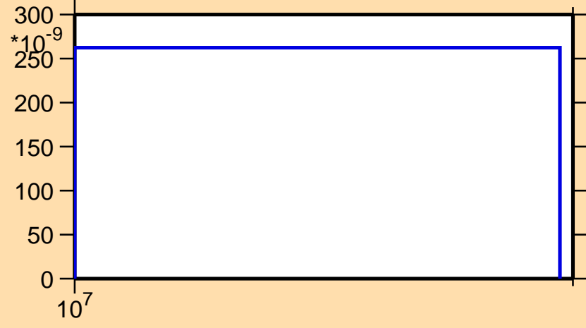
\sigma vs. E for ^{125}\text{Pr}(n,\text{pt})
