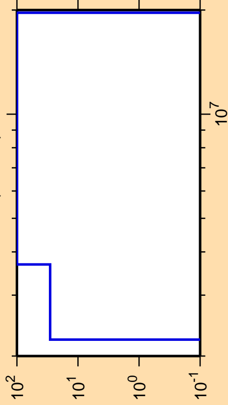
\Delta\sigma/\sigma vs. E for ^{125}\text{Pr}(n,\text{He}3)
