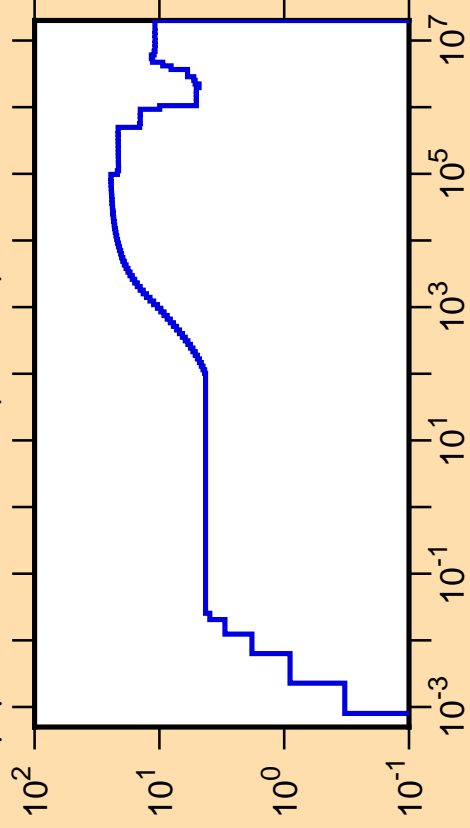
\Delta\mu/\mu vs. E for ^{126}\text{Pr}(\text{mt251})
