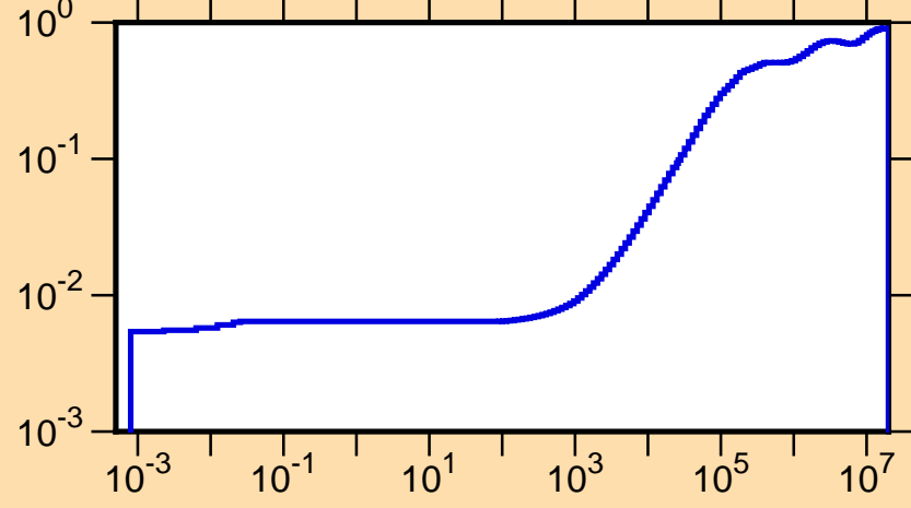
\mu vs. E for ^{126}\text{Pr}(\text{mt251})
