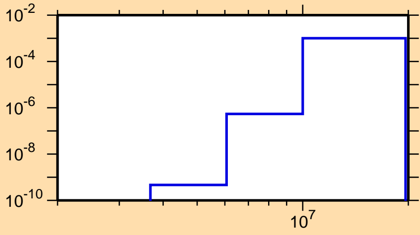
\sigma vs. E for ^{126}\text{Pr}(n,\text{He3})
