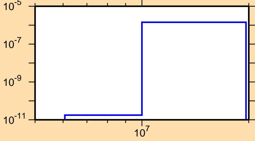
\sigma vs. E for ^{126}\text{Pr}(\text{mt117})
