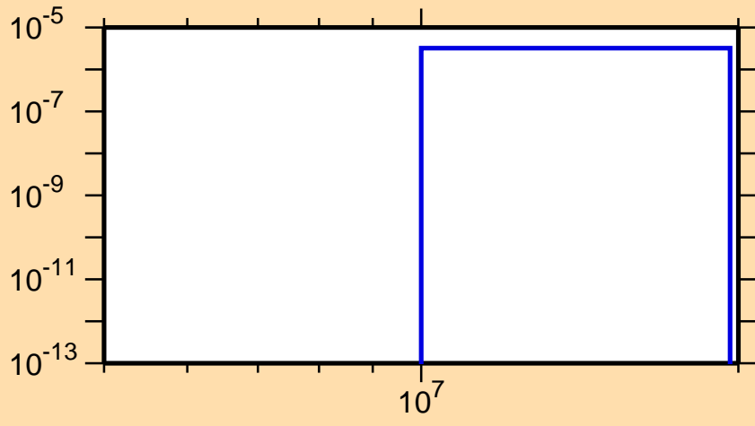
\sigma vs. E for ^{126}\text{Pr}(n,nd)
