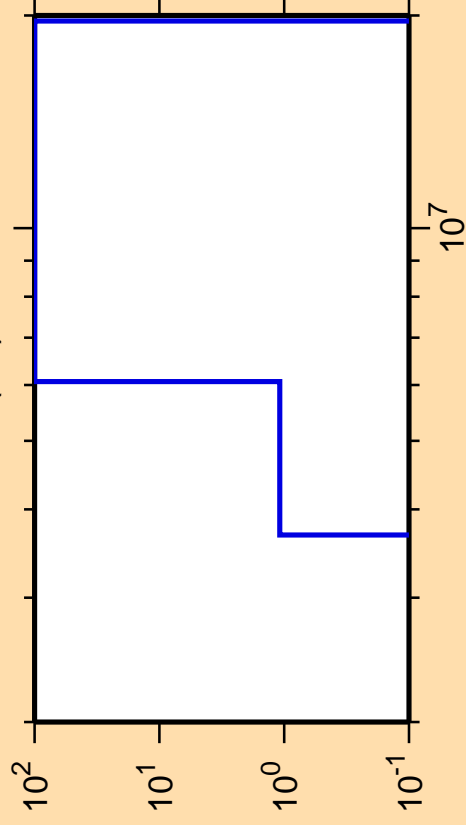
\Delta\sigma/\sigma vs. E for ^{126}\text{Pr}(n,t)
