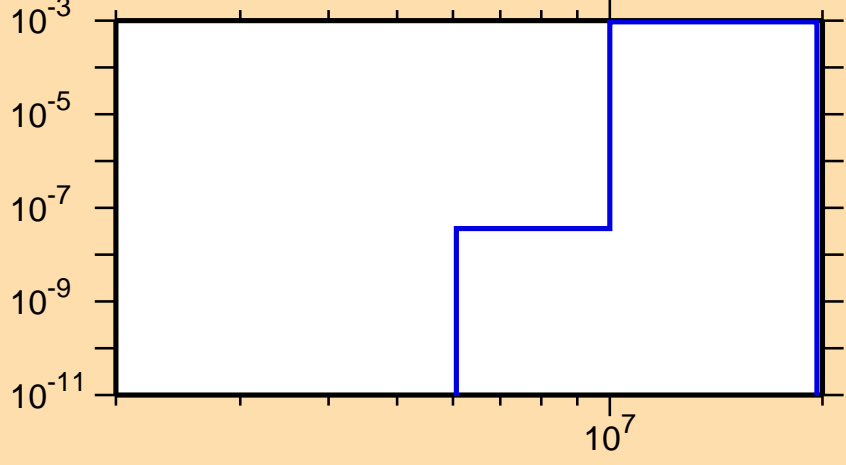
\sigma vs. E for ^{126}\text{Pr}(n,t)
