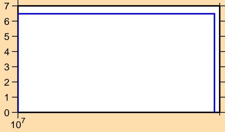
\Delta\sigma/\sigma vs. E for ^{126}\text{Pr}(n,\text{tot.})
