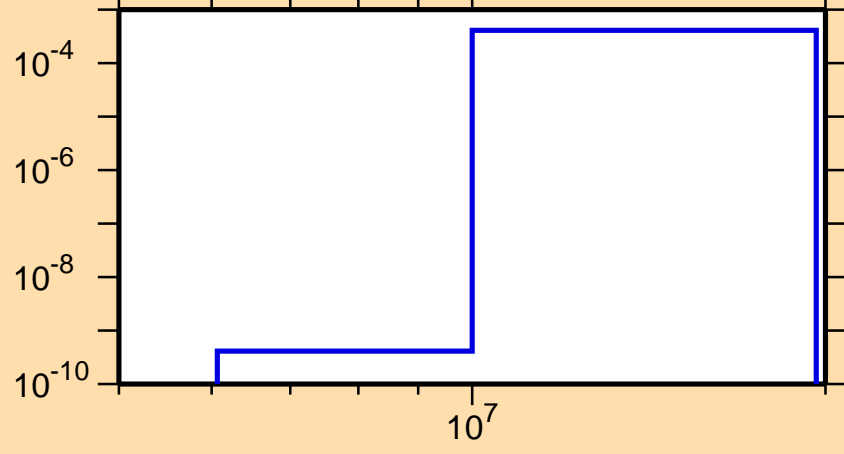
\sigma vs. E for ^{126}\text{Pr}(n,\text{pd})
