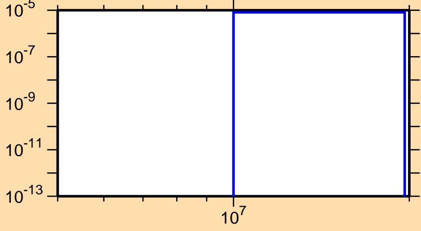
\sigma vs. E for ^{126}\text{Pr}(n,\text{pt})
