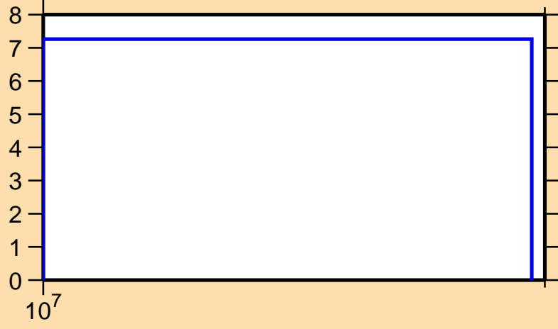
\Delta\sigma/\sigma vs. E for ^{126}\text{Pr}(n,\text{nonel.})
