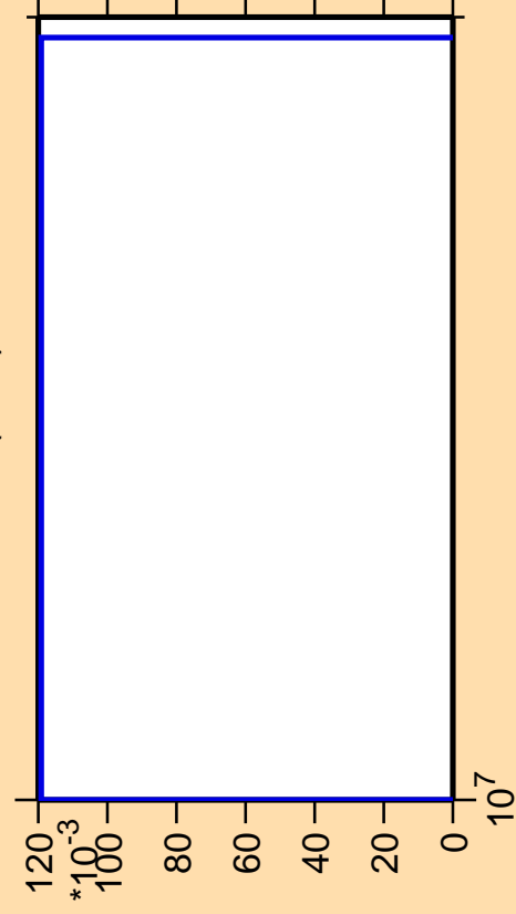
\Delta\sigma/\sigma vs. E for ^{126}\text{Pr}(n,nt)
