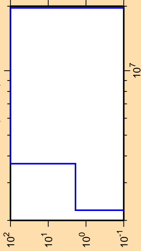
\Delta\sigma/\sigma vs. E for ^{126}\text{Pr}(n,\text{He3})
