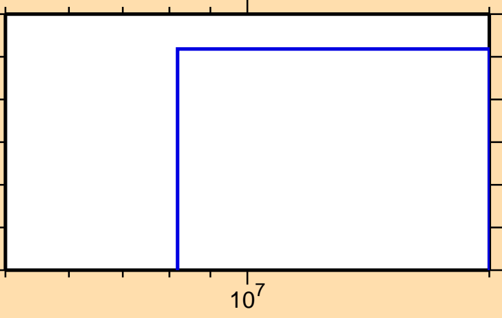
\sigma vs. E for ^{126}\text{Pr}(n,\text{nd})
