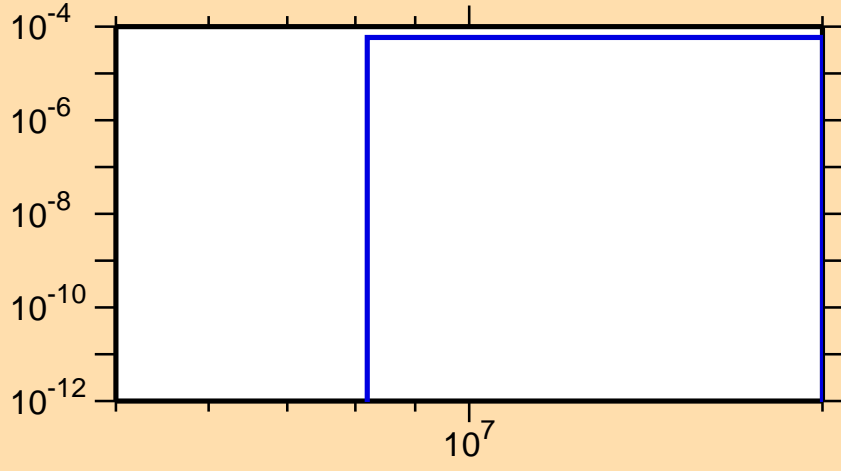
\sigma vs. E for ^{126}\text{Pr}(\text{mt } 45)
