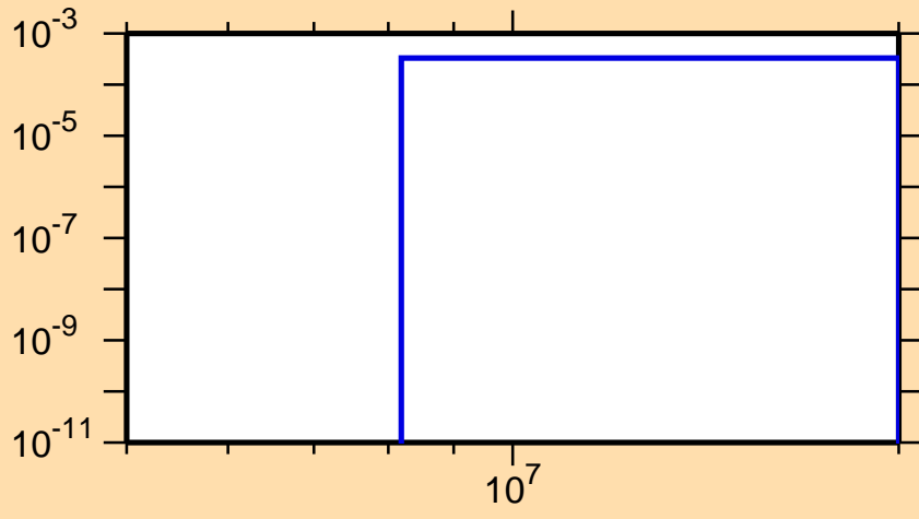
\sigma vs. E for ^{126}\text{Pr}(n,\text{pd})
