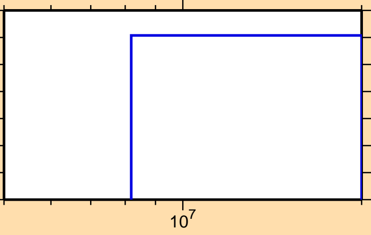
\sigma vs. E for ^{126}\text{Pr}(n,2n)
