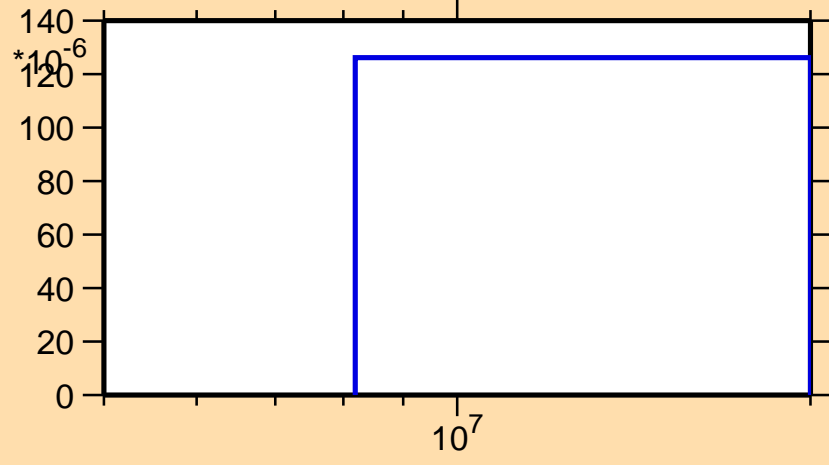
\sigma vs. E for ^{126}\text{Pr}(n,2np)
