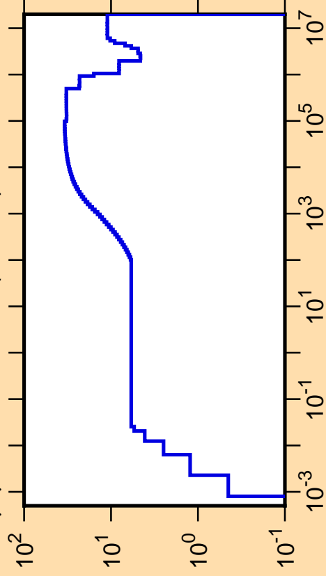
\Delta\mu/\mu vs. E for ^{127}\text{Pr}(\text{mt251})
