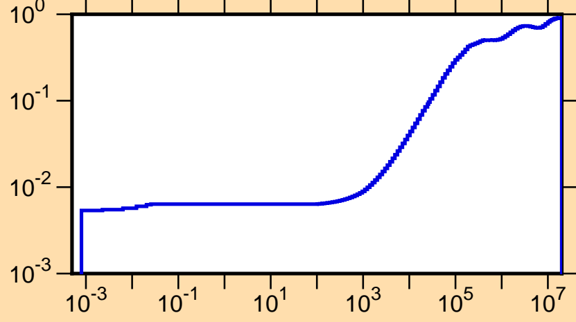
\mu vs. E for ^{127}\text{Pr}(\text{mt251})
