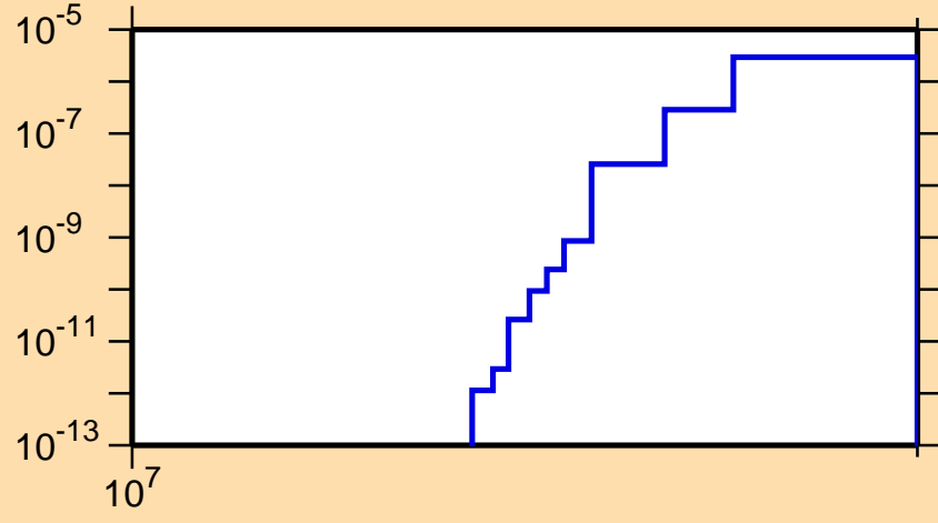
\sigma vs. E for ^{127}\text{Pr}(n,nd)
