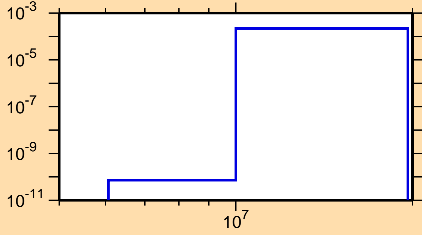
\sigma vs. E for ^{127}\text{Pr}(n,\text{pd})
