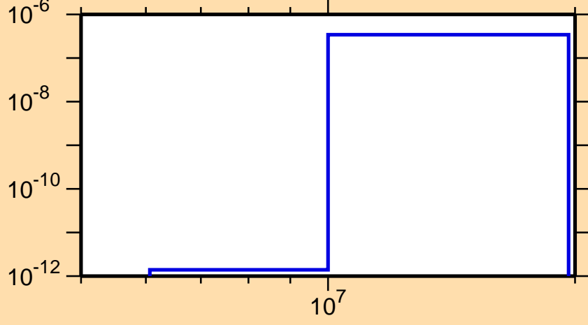
\sigma vs. E for ^{127}\text{Pr}(\text{mt117})
