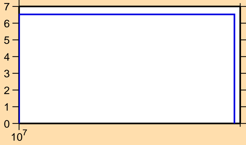
\Delta\sigma/\sigma vs. E for ^{127}\text{Pr}(n,\text{nonel.})
