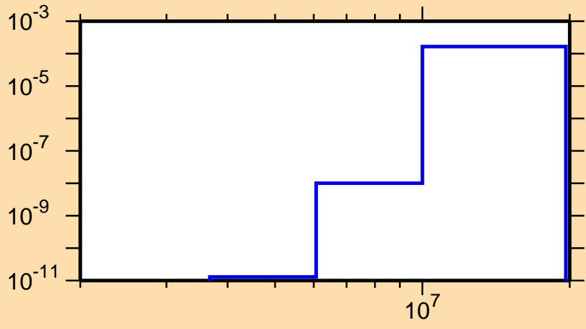
\sigma vs. E for ^{127}\text{Pr}(n,\text{He}3)
