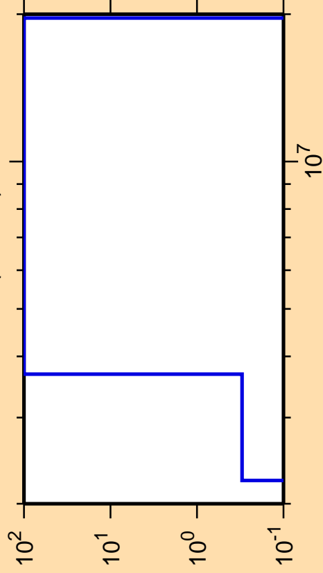
\Delta\sigma/\sigma vs. E for ^{127}\text{Pr}(n,\text{He}3)
