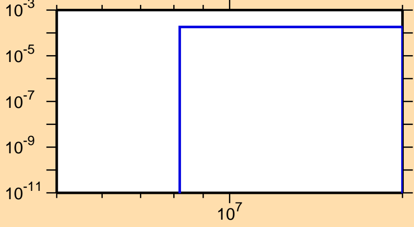
\sigma vs. E for ^{127}\text{Pr}(n,t)
