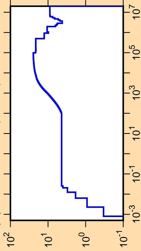
\Delta\mu/\mu vs. E for ^{128}\text{Pr}(\text{mt251})
