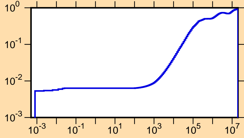
\mu vs. E for ^{128}\text{Pr}(\text{mt251})
