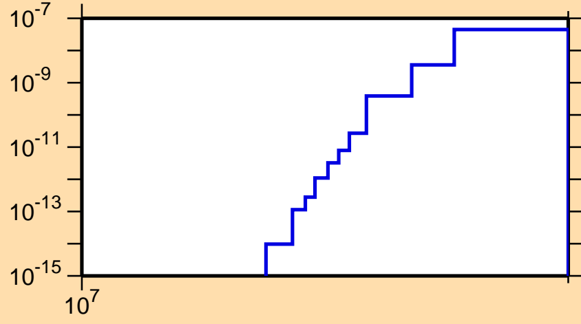
\sigma vs. E for ^{128}\text{Pr}(n,2n\alpha)
