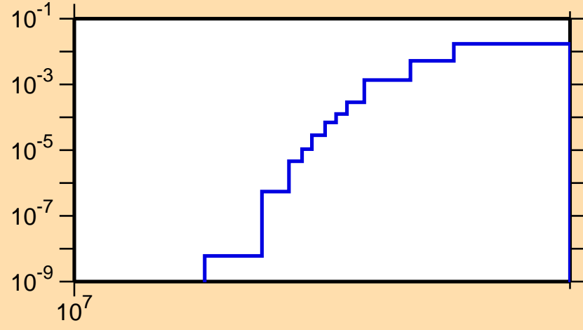
\sigma vs. E for ^{128}\text{Pr}(n,2np)
