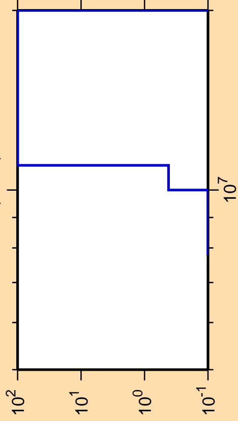
\Delta\sigma/\sigma vs. E for ^{128}\text{Pr}(n,nd)
