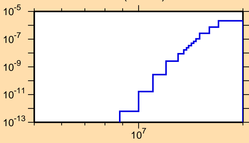
\sigma vs. E for ^{128}\text{Pr}(\text{mt117})
