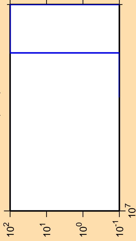
\Delta\sigma/\sigma vs. E for ^{128}\text{Pr}(n,nt)
