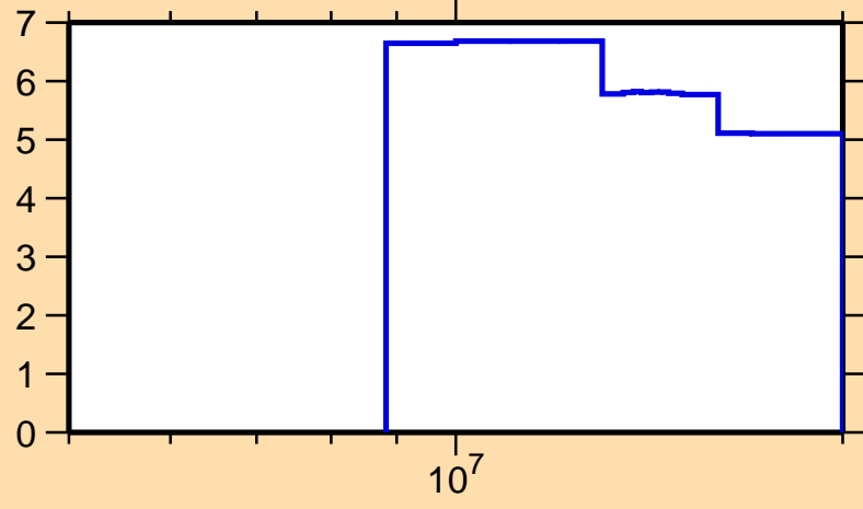
\Delta\sigma/\sigma vs. E for ^{128}\text{Pr}(n,\text{nonel.})
