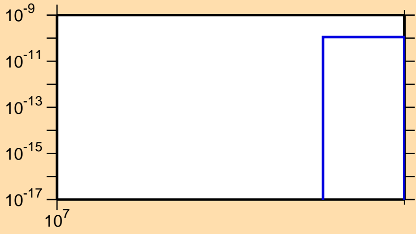
\sigma vs. E for ^{128}\text{Pr}(n,nt)
