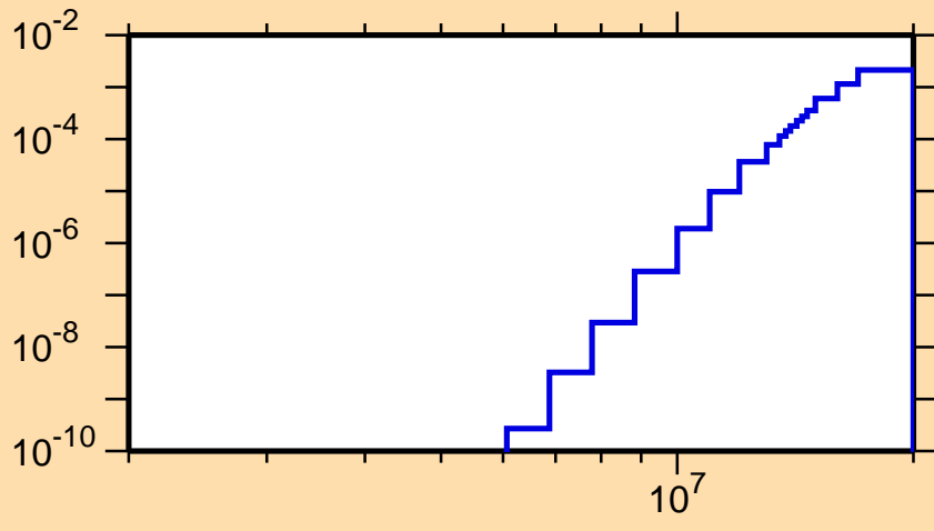
\sigma vs. E for ^{128}\text{Pr}(n,\text{He3})
