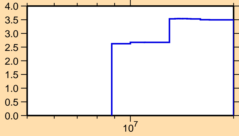
\Delta\sigma/\sigma vs. E for ^{128}\text{Pr}(n,\text{tot.})
