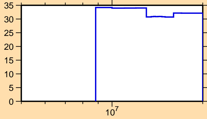
\Delta\sigma/\sigma vs. E for ^{128}\text{Pr}(n,\text{inel.})
