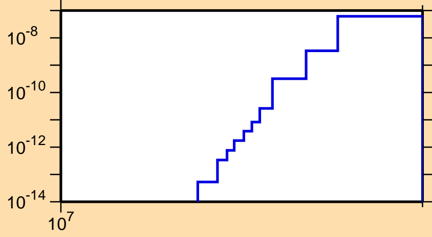
\sigma vs. E for ^{128}\text{Pr}(\text{mt } 34)
