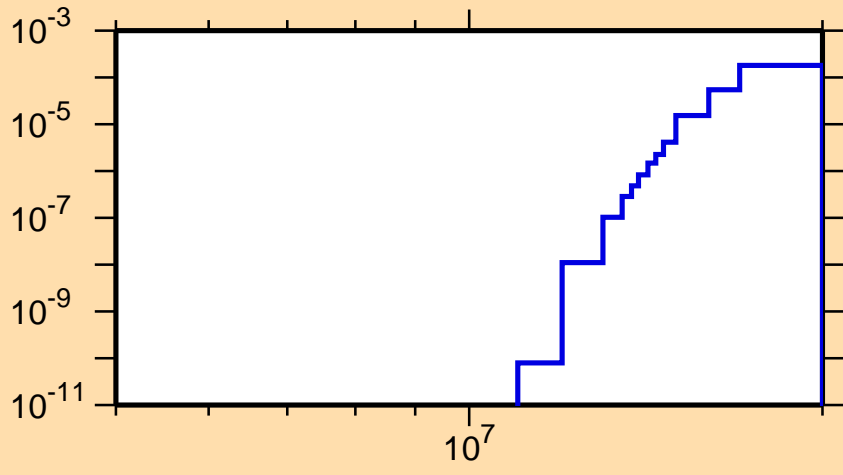
\sigma vs. E for ^{128}\text{Pr}(n,nd)
