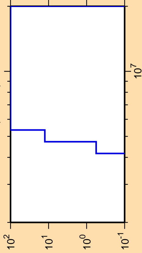
\Delta\sigma/\sigma vs. E for ^{128}\text{Pr}(n,\text{He3})
