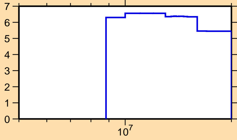
\Delta\sigma/\sigma vs. E for ^{128}\text{Pr}(n,\text{el.})
