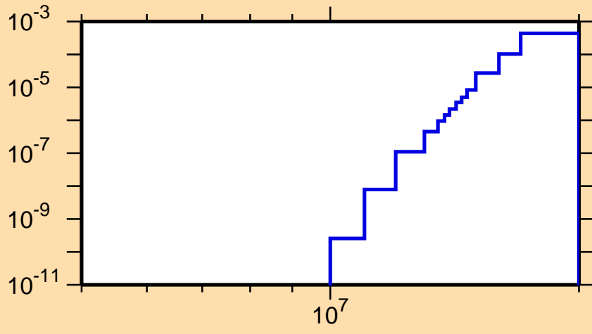
\sigma vs. E for ^{128}\text{Pr}(\text{mt } 45)
