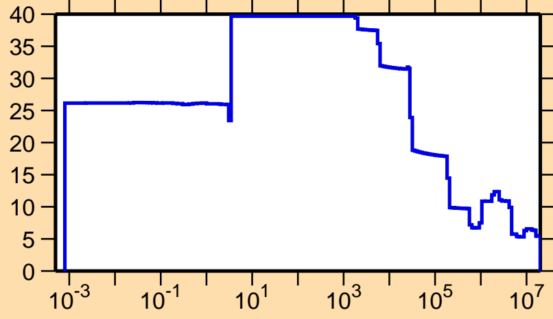
\Delta\sigma/\sigma vs. E for ^{128}\text{Pr}(n,\text{el.})
