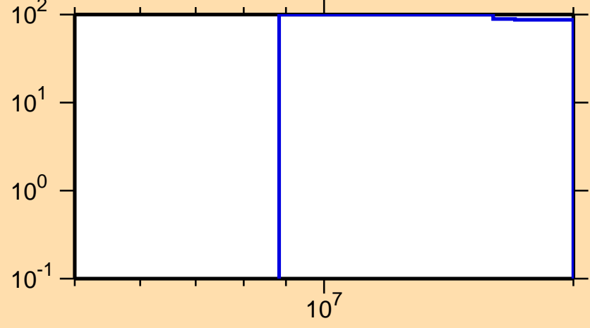
\Delta\sigma/\sigma vs. E for ^{128}\text{Pr}(n,2n)
