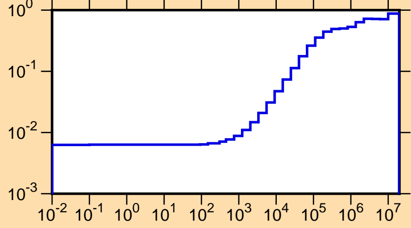
\mu vs. E for ^{128}\text{Pr}(\text{mt251})
