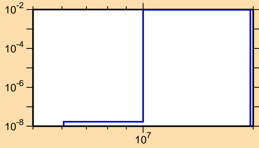
\sigma vs. E for ^{128}\text{Pr}(n,2n)
