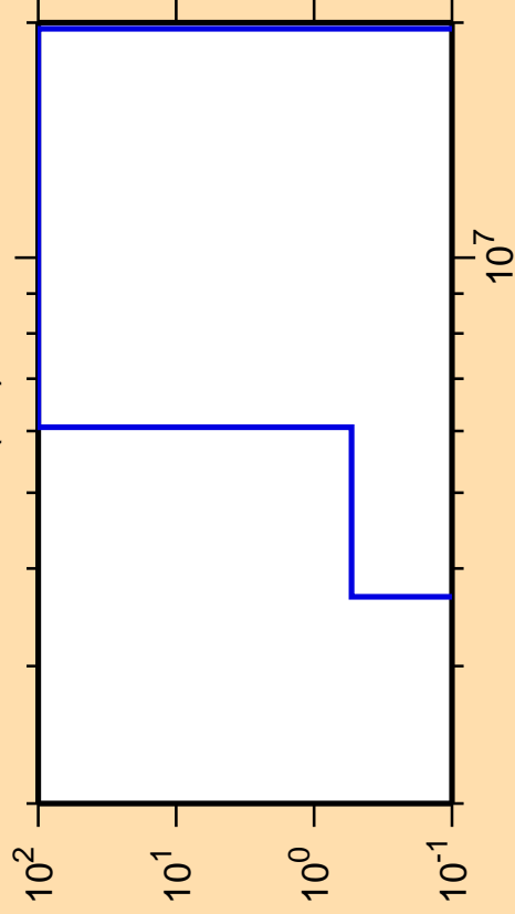
\Delta\sigma/\sigma vs. E for ^{128}\text{Pr}(n,t)
