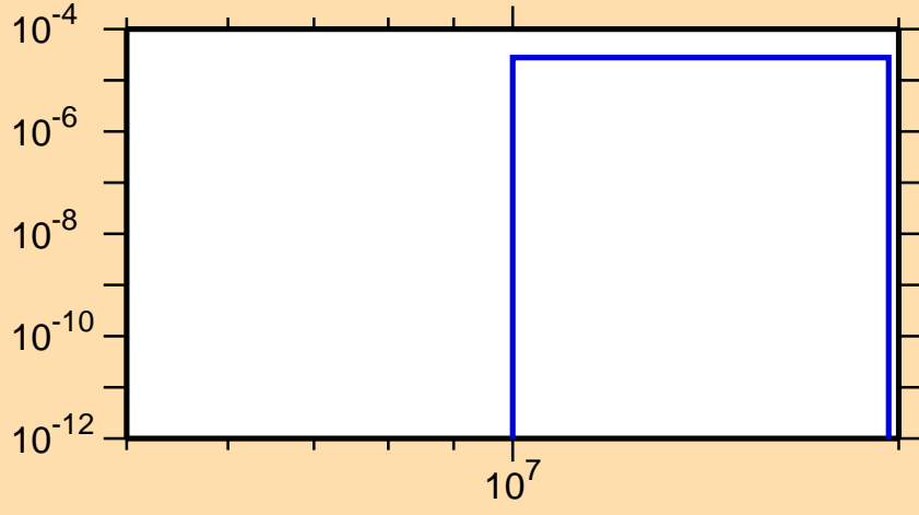
\sigma vs. E for ^{128}\text{Pr}(n,\text{pd})
