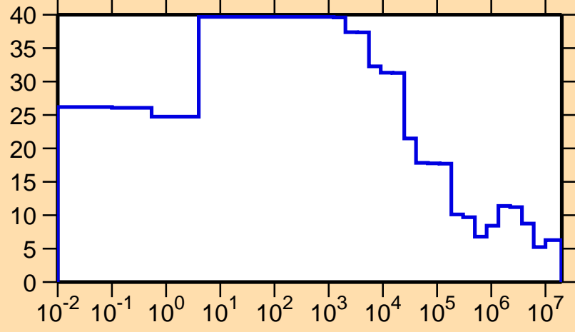
\Delta\sigma/\sigma vs. E for ^{128}\text{Pr}(n,el.)
