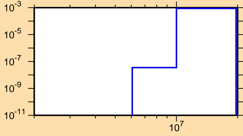
\sigma vs. E for ^{128}\text{Pr}(n,t)
