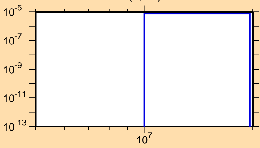
\sigma vs. E for ^{128}\text{Pr}(n,\text{nd})
