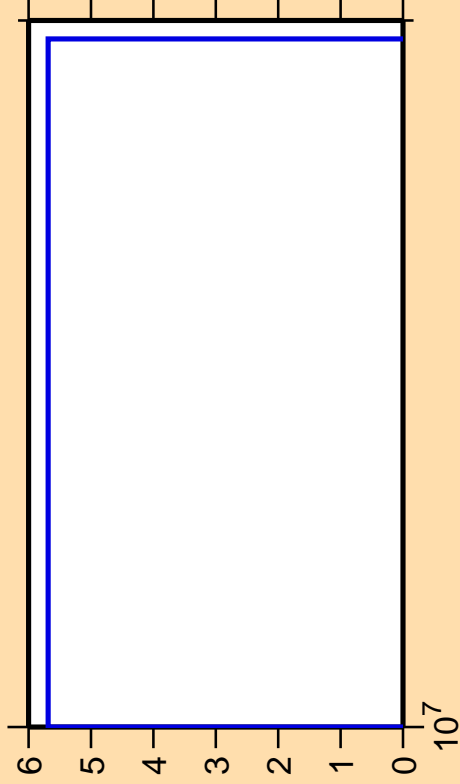
\Delta\sigma/\sigma vs. E for ^{128}\text{Pr}(n,nt)
