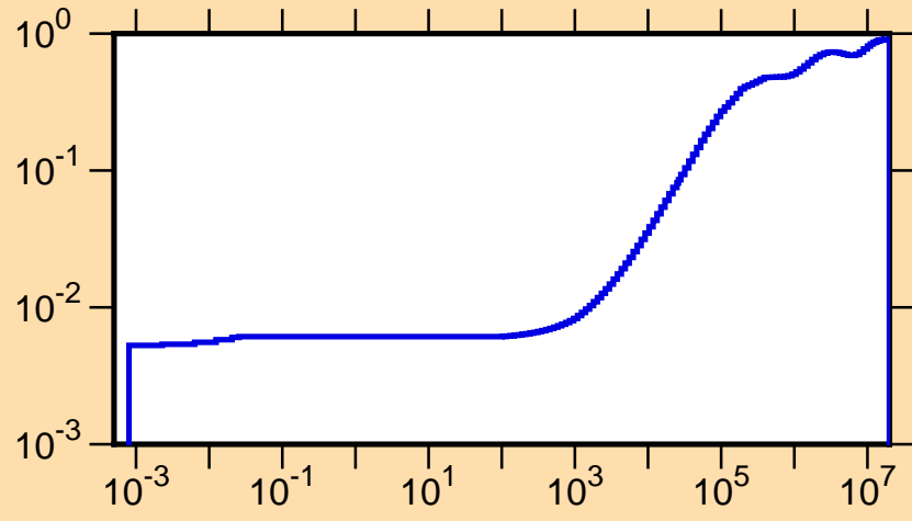
\mu vs. E for ^{129}\text{Pr}(\text{mt251})
