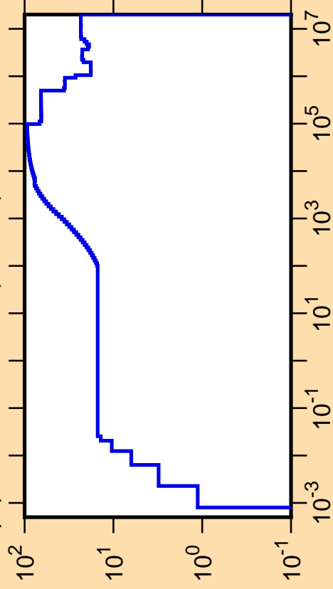
\Delta\mu/\mu vs. E for ^{129}\text{Pr}(\text{mt251})
