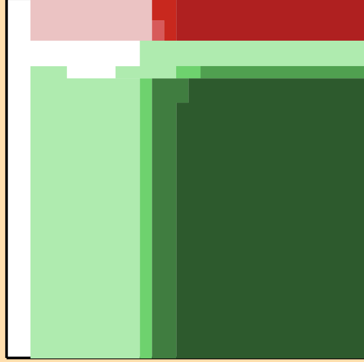
\Delta\sigma/\sigma vs. E for ^{129}\text{Pr}(n,ncont.)
