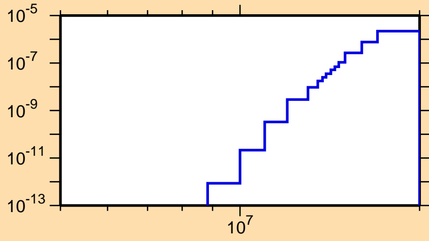
\sigma vs. E for ^{129}\text{Pr}(\text{mt117})
