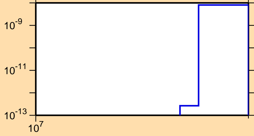
\sigma vs. E for ^{129}\text{Pr}(n,nt)
