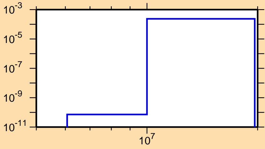
\sigma vs. E for ^{129}\text{Pr}(n,t)
