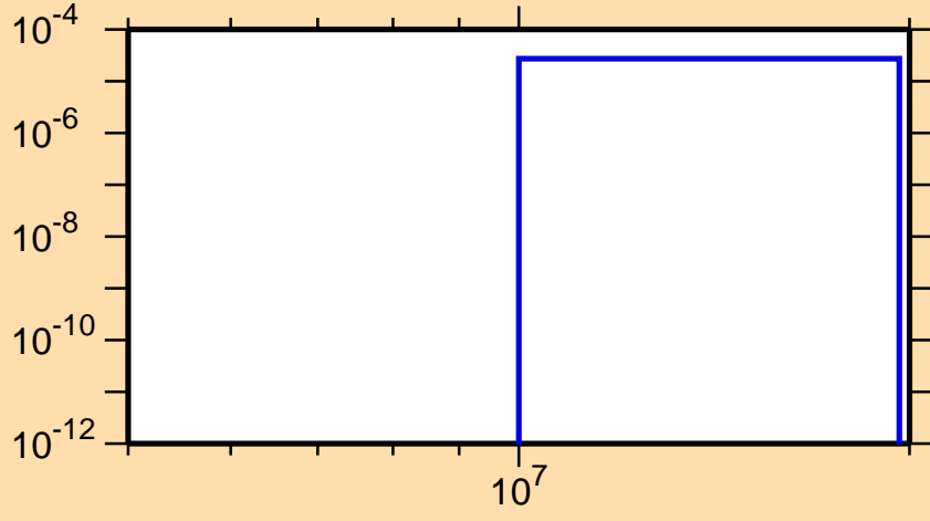
\sigma vs. E for ^{129}\text{Pr}(n,\text{pd})
