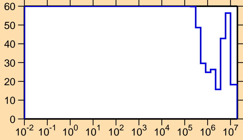
\Delta\sigma/\sigma vs. E for ^{129}\text{Pr}(n,el.)
