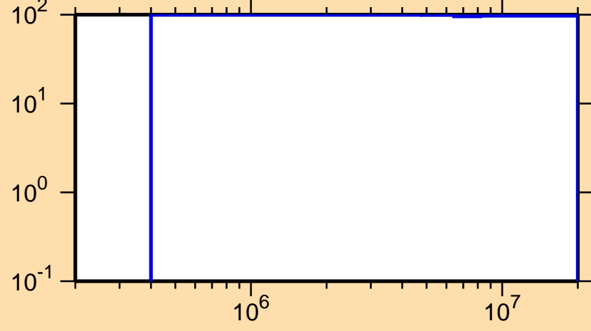
\Delta\sigma/\sigma vs. E for ^{129}\text{Pr}(n,n\text{cont.})
