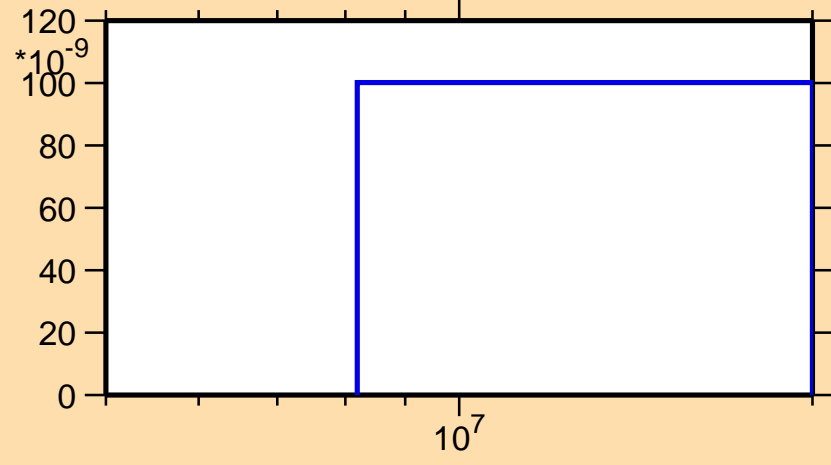
\sigma vs. E for ^{129}\text{Pr}(\text{mt117})
