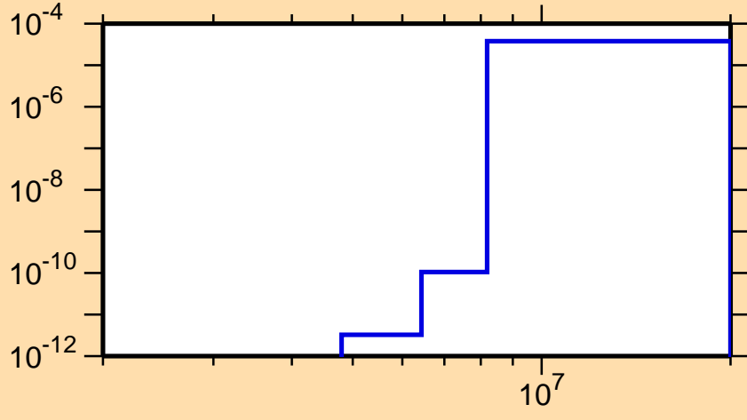
\sigma vs. E for ^{129}\text{Pr}(n,\text{He3})
