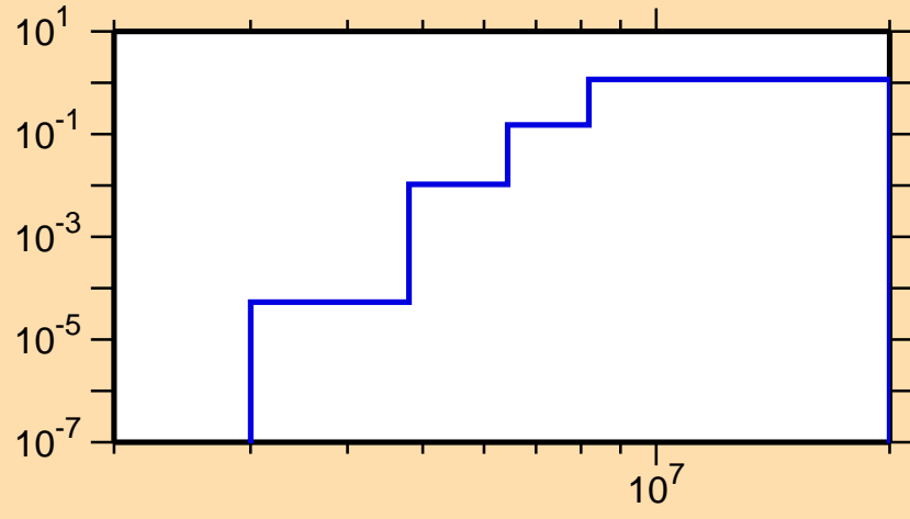
\sigma vs. E for ^{129}\text{Pr}(n,np)
