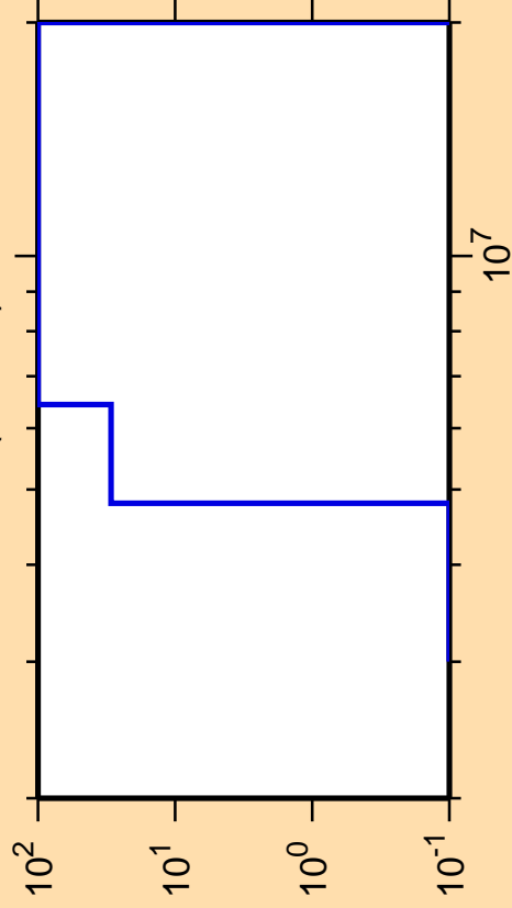
\Delta\sigma/\sigma vs. E for ^{129}\text{Pr}(n,\text{He3})
