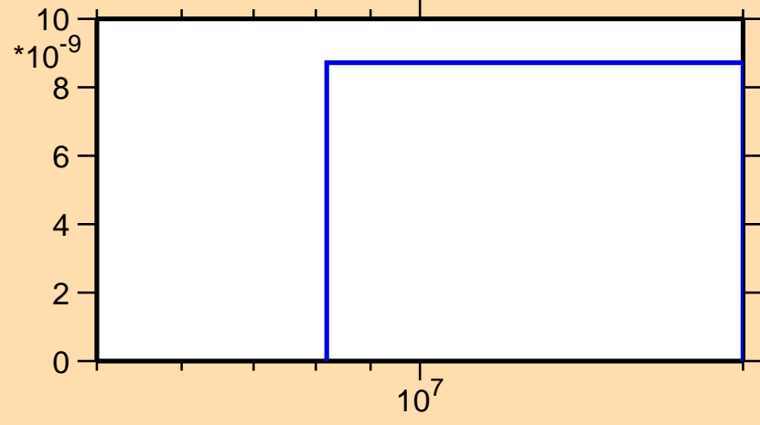
\sigma vs. E for ^{130}\text{Pr}(\text{mt117})
