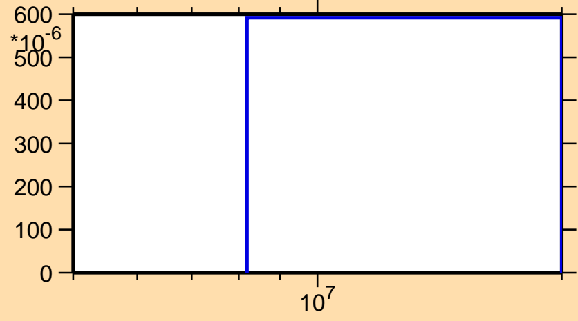
\sigma vs. E for ^{130}\text{Pr}(n,2np)
