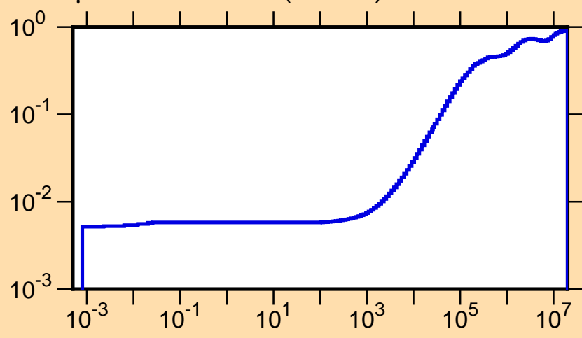
\mu vs. E for ^{131}\text{Pr}(\text{mt251})
