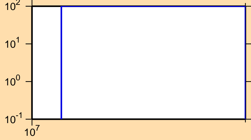
\Delta\sigma/\sigma vs. E for ^{131}\text{Pr}(n,2n)
