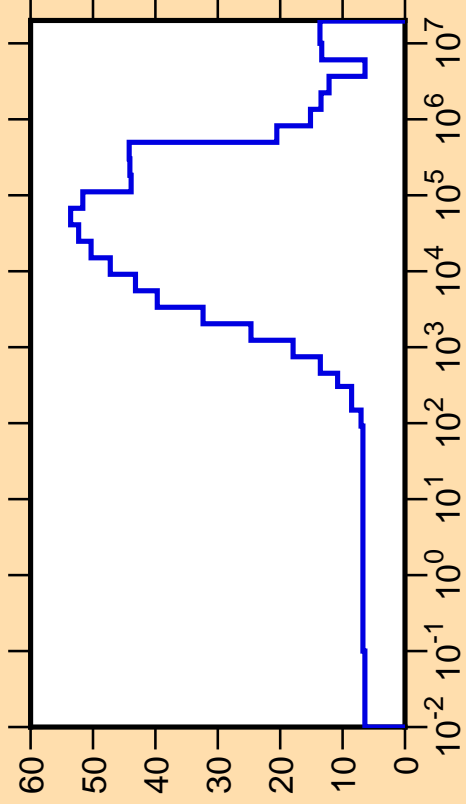
\Delta\mu/\mu vs. E for ^{131}\text{Pr}(\text{mt251})
