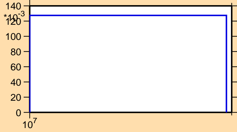
\sigma vs. E for ^{131}\text{Pr}(n,2n)
