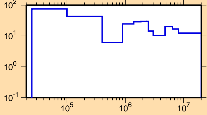
\Delta\sigma/\sigma vs. E for ^{131}\text{Pr}(n,\text{el.})
