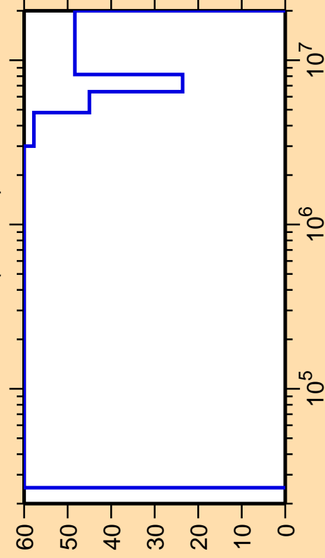
\Delta\sigma/\sigma vs. E for ^{131}\text{Pr}(n,\text{inel.})
