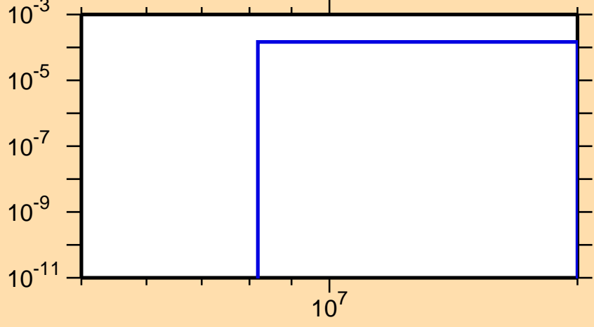
\sigma vs. E for ^{131}\text{Pr}(n,t)
