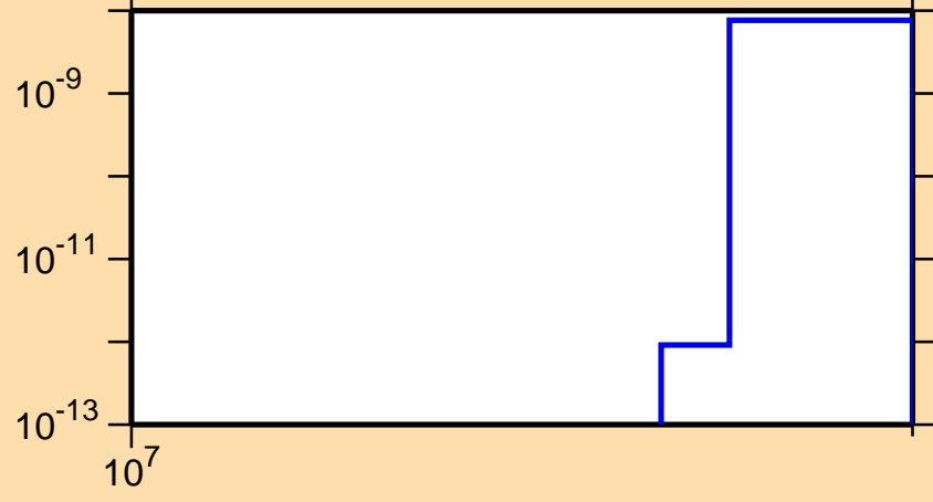
\sigma vs. E for ^{131}\text{Pr}(n,nt)
