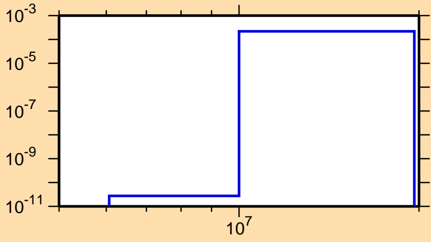
\sigma vs. E for ^{131}\text{Pr}(n,t)
