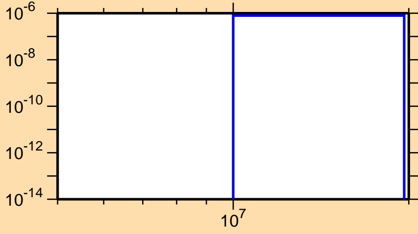
\sigma vs. E for ^{131}\text{Pr}(n,\text{pd})
