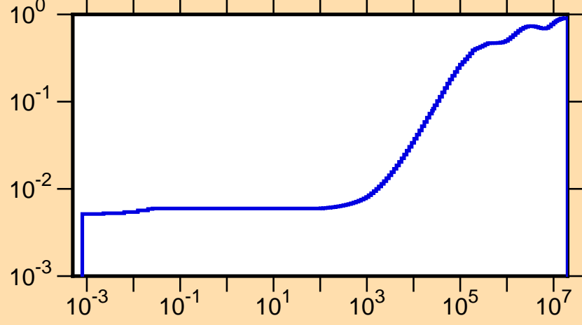
\mu vs. E for ^{132}\text{Pr}(\text{mt251})
