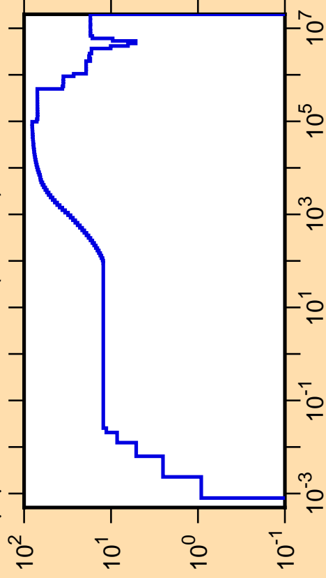
\Delta\mu/\mu vs. E for ^{132}\text{Pr}(\text{mt251})
