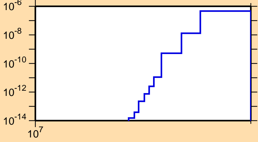
\sigma vs. E for ^{132}\text{Pr}(n,\text{pt})
