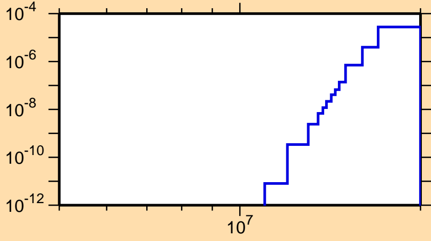
\sigma vs. E for ^{132}\text{Pr}(\text{mt } 45)
