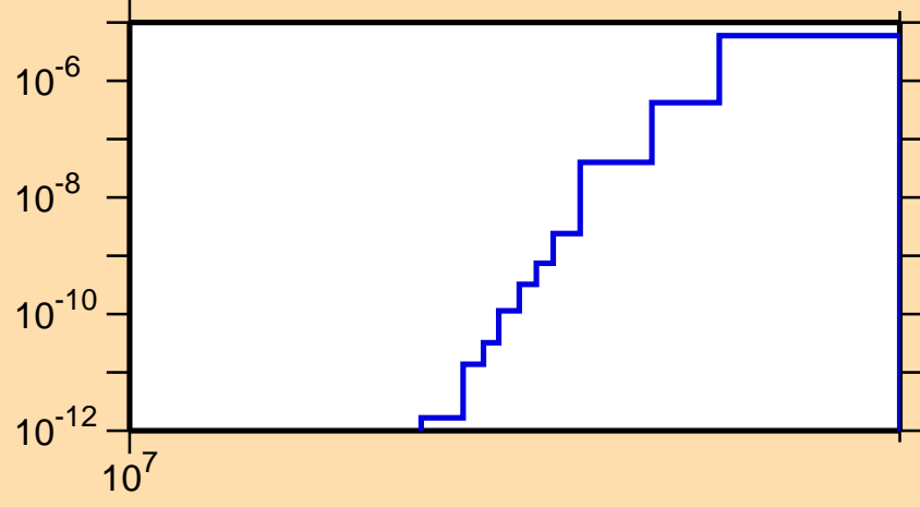
\sigma vs. E for ^{132}\text{Pr}(n,2n\alpha)
