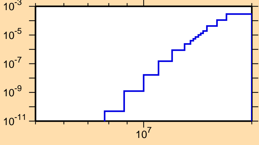
\sigma vs. E for ^{132}\text{Pr}(n,\text{He}3)
