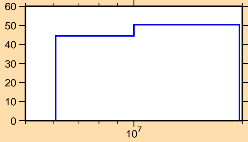
\Delta\sigma/\sigma vs. E for ^{132}\text{Pr}(n,\text{inel.})
