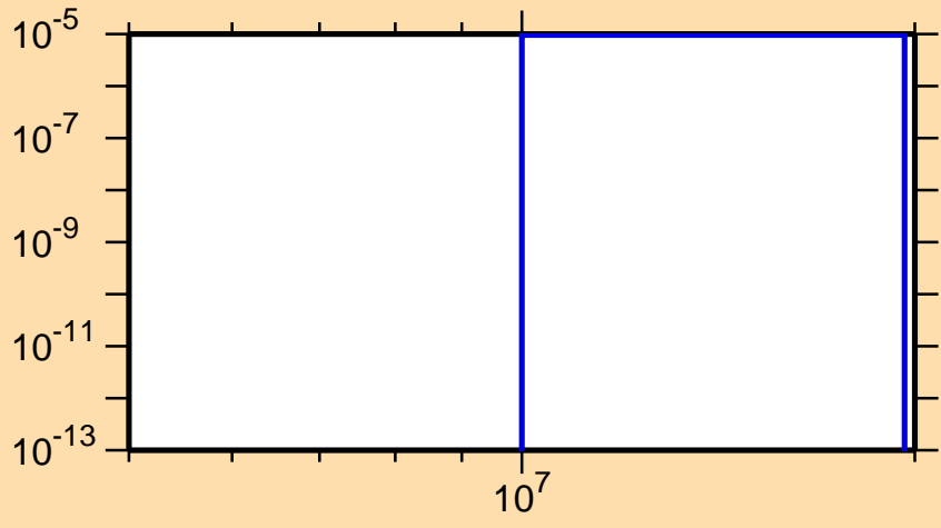
\sigma vs. E for ^{132}\text{Pr}(n,\text{nd})
