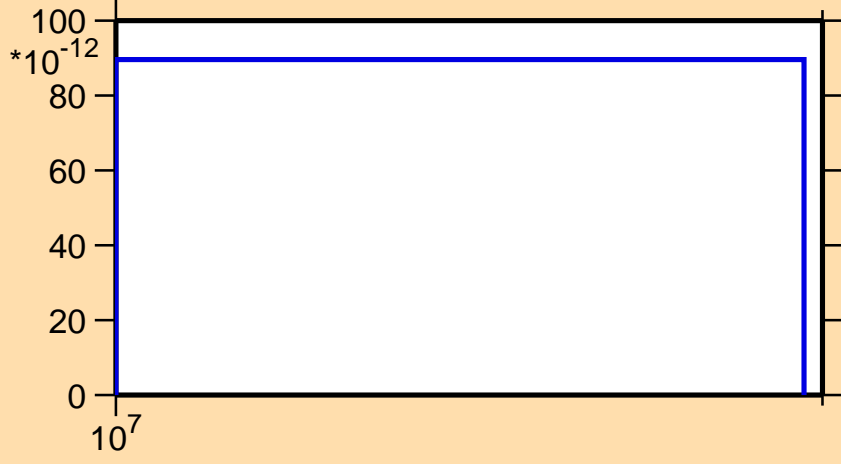
\sigma vs. E for ^{132}\text{Pr}(n,nt)
