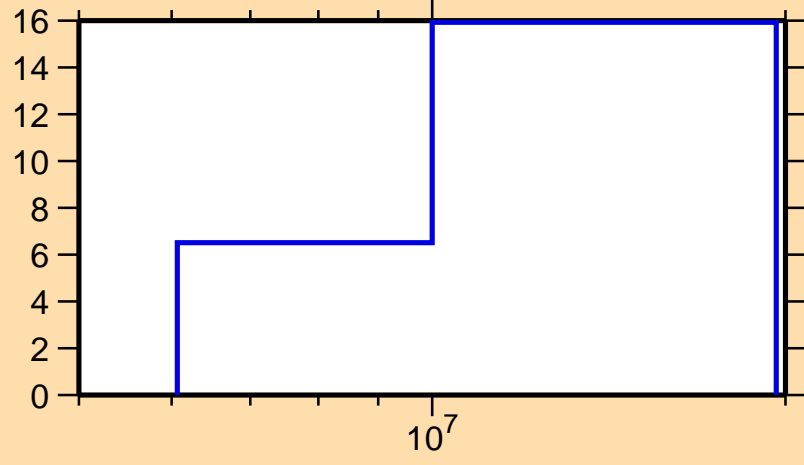
\Delta\sigma/\sigma vs. E for ^{132}\text{Pr}(n,\text{tot.})
