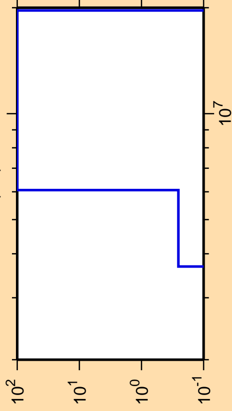
\Delta\sigma/\sigma vs. E for ^{132}\text{Pr}(n,t)
