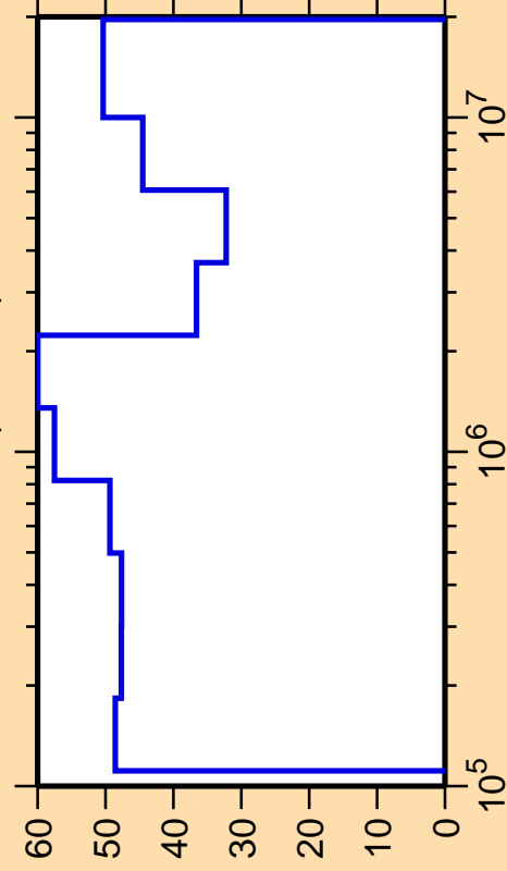
\Delta\sigma/\sigma vs. E for ^{132}\text{Pr}(n,\text{inel.})
