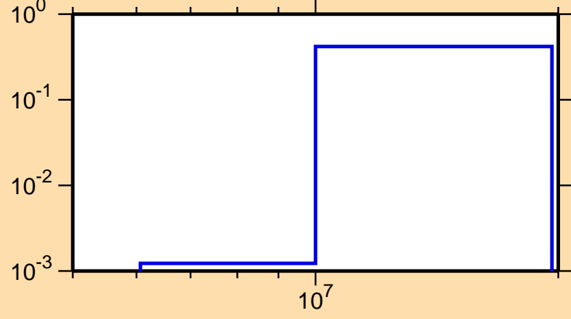
\sigma vs. E for ^{132}\text{Pr}(n,2n)
