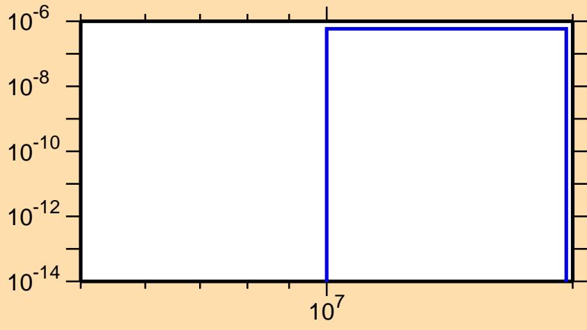
\sigma vs. E for ^{132}\text{Pr}(\text{mt } 45)
