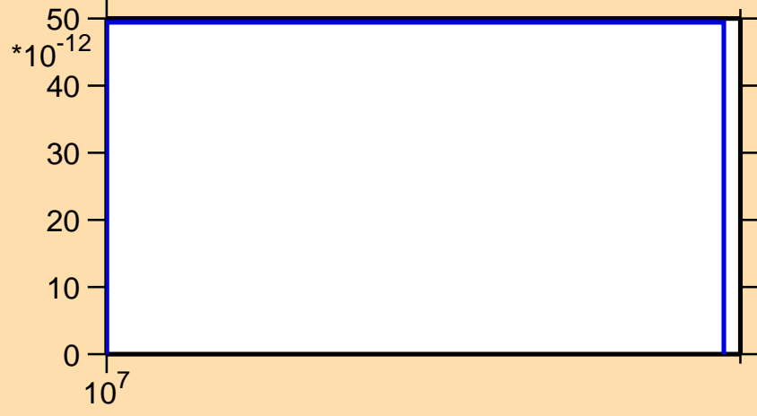
\sigma vs. E for ^{132}\text{Pr}(\text{mt } 34)
