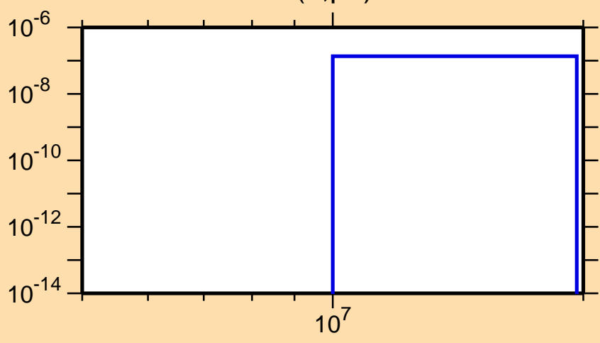
\sigma vs. E for ^{132}\text{Pr}(n,\text{pd})
