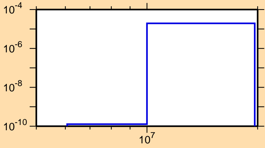
\sigma vs. E for ^{132}\text{Pr}(n,\text{He3})
