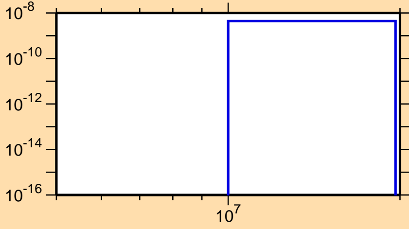
\sigma vs. E for ^{132}\text{Pr}(\text{mt117})
