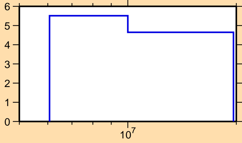
\Delta\sigma/\sigma vs. E for ^{132}\text{Pr}(n,\text{nonel.})
