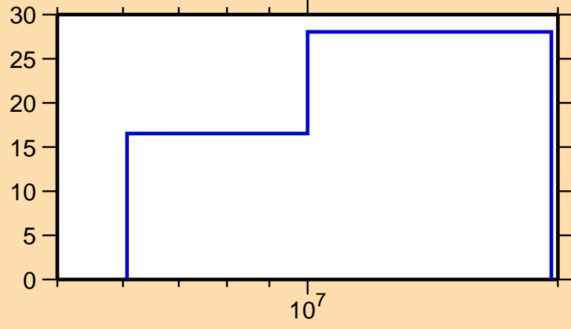
\Delta\sigma/\sigma vs. E for ^{132}\text{Pr}(n,\text{el.})
