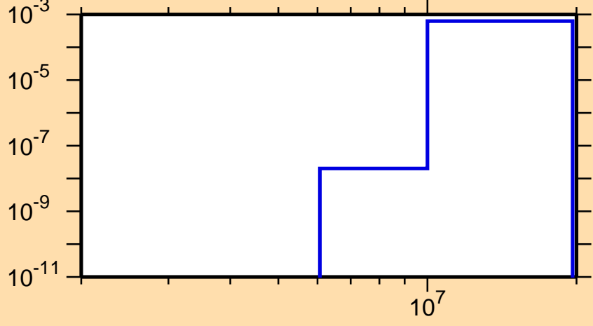
\sigma vs. E for ^{132}\text{Pr}(n,t)
