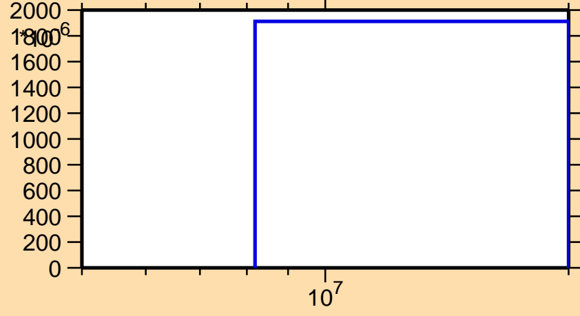
\sigma vs. E for ^{132}\text{Pr}(n,2np)
