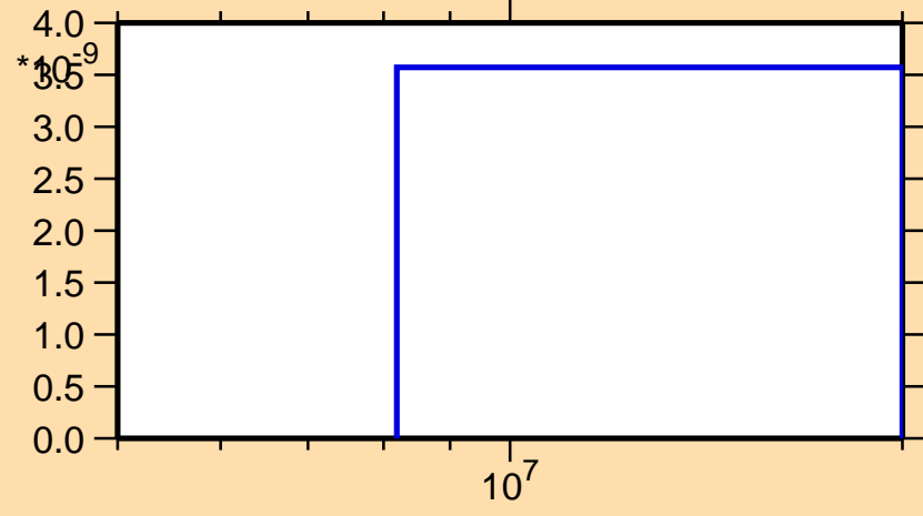
\sigma vs. E for ^{132}\text{Pr}(\text{mt117})
