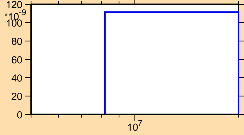
\sigma vs. E for ^{132}\text{Pr}(n,\text{pd})
