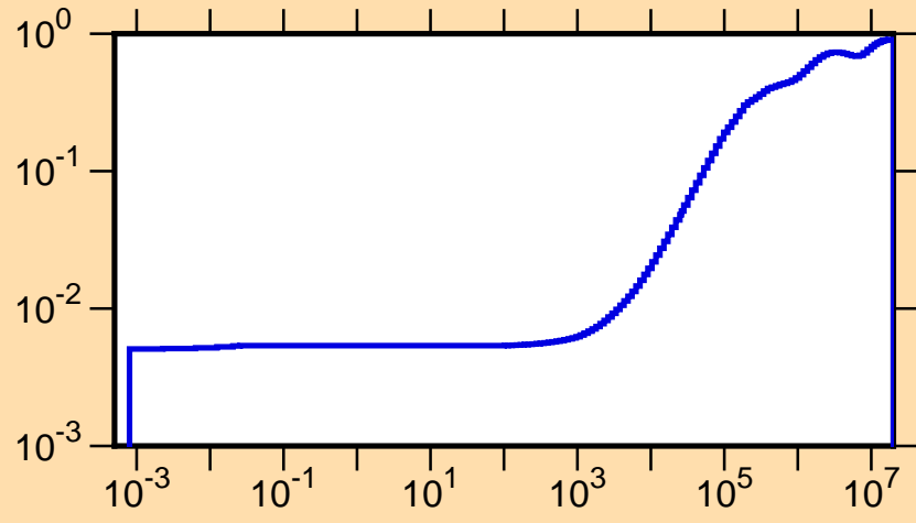
\mu vs. E for ^{133}\text{Pr}(\text{mt251})
