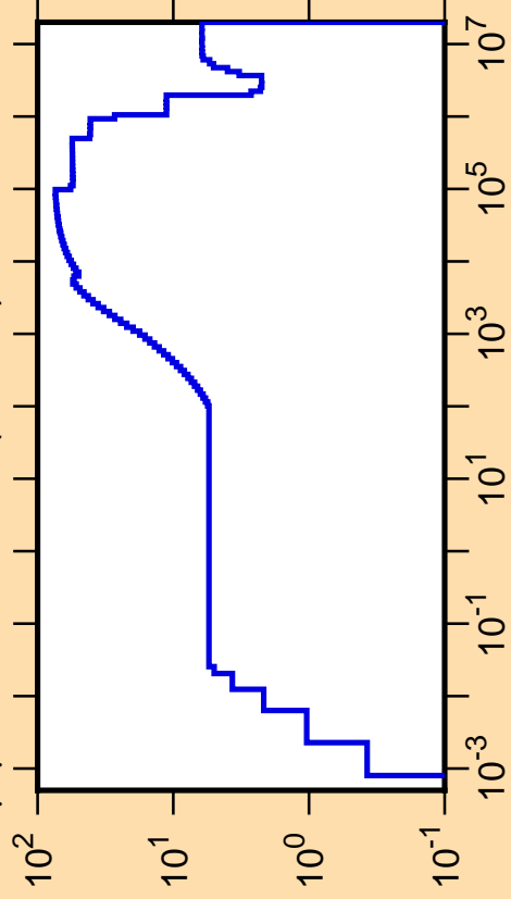
\Delta\mu/\mu vs. E for ^{133}\text{Pr}(\text{mt251})
