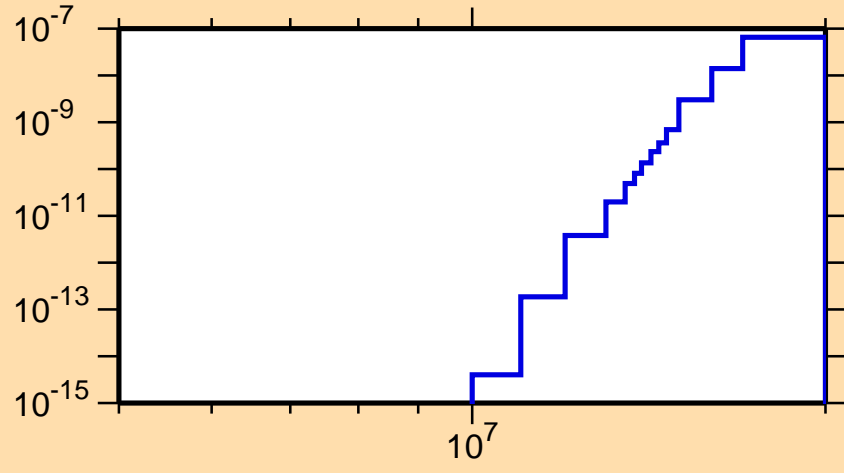
\sigma vs. E for ^{133}\text{Pr}(\text{mt117})
