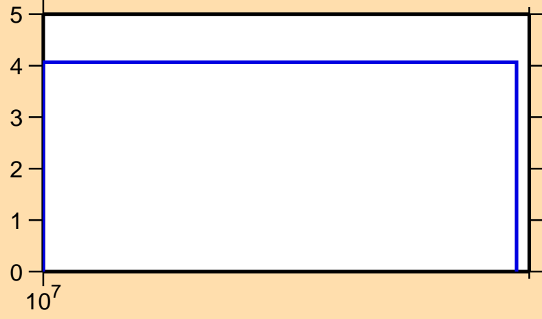
\Delta\sigma/\sigma vs. E for ^{133}\text{Pr}(n,el.)
