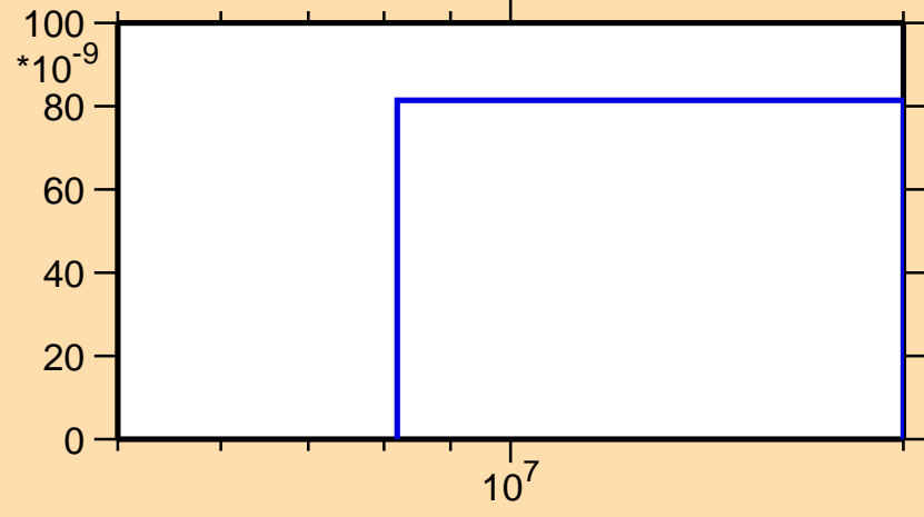
\sigma vs. E for ^{133}\text{Pr}(n,pd)
