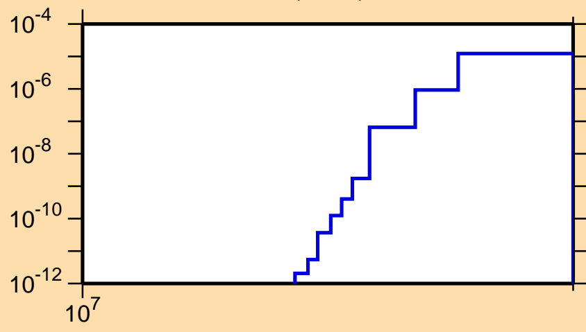
\sigma vs. E for ^{133}\text{Pr}(n,nd)
