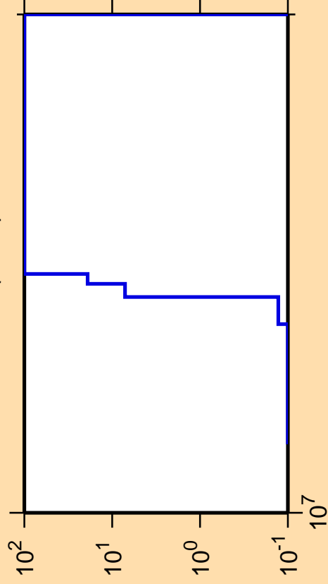
\Delta\sigma/\sigma vs. E for ^{133}\text{Pr}(n,nd)
