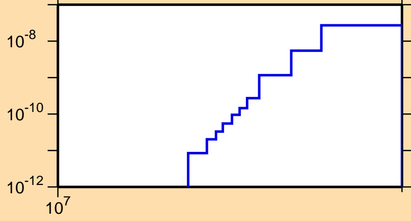
\sigma vs. E for ^{133}\text{Pr}(\text{mt117})
